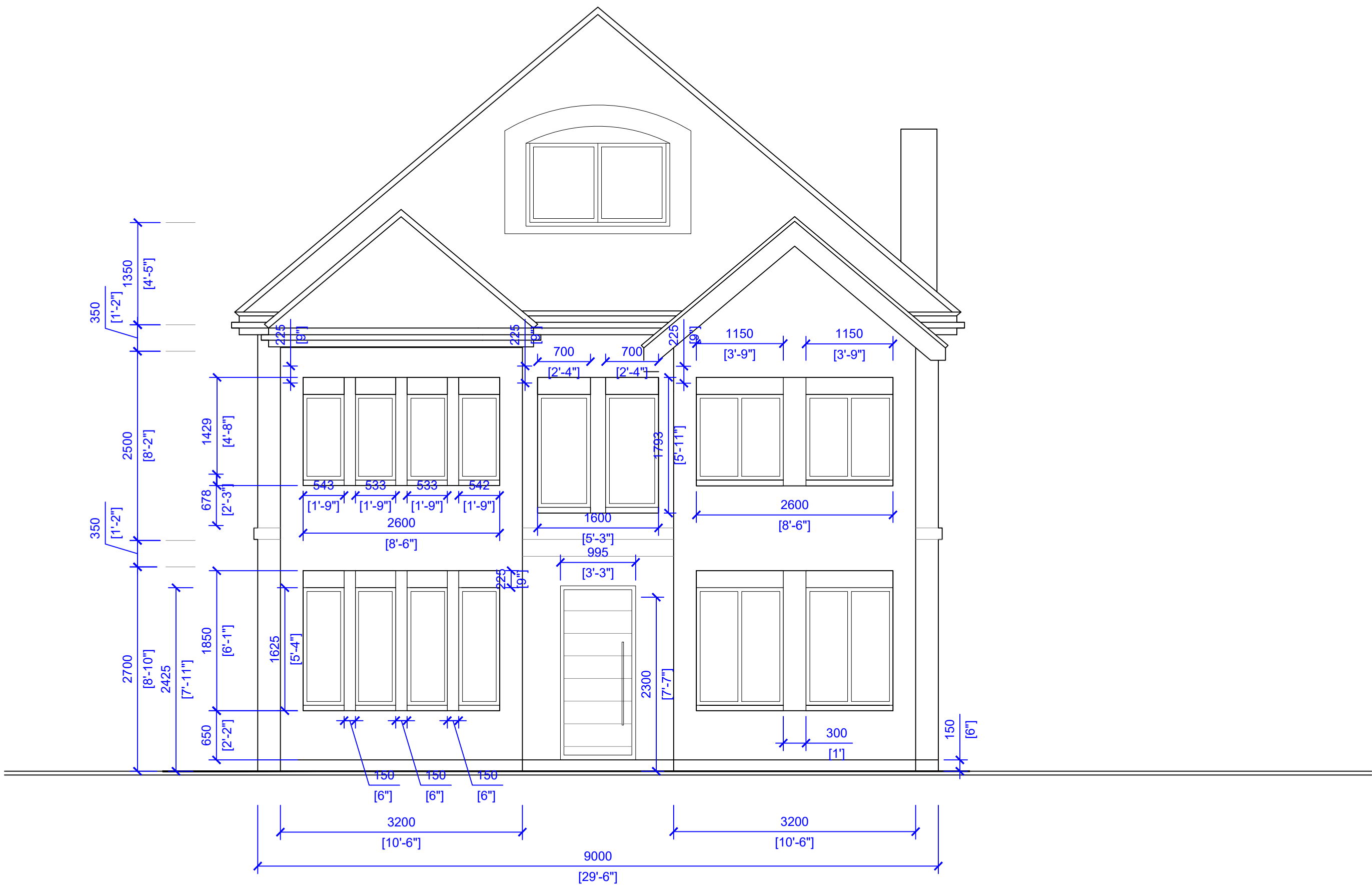
PROPOSED FRONT ELEVATION 1:100
