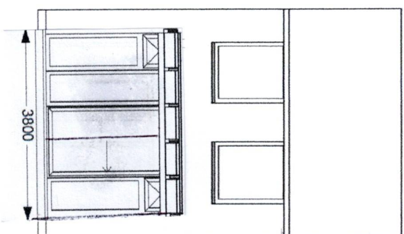
Existing Rear Elevation 1:100
