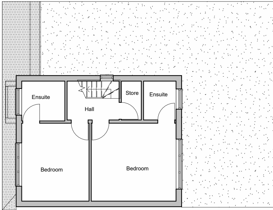
1 First Floor 1 : 100
