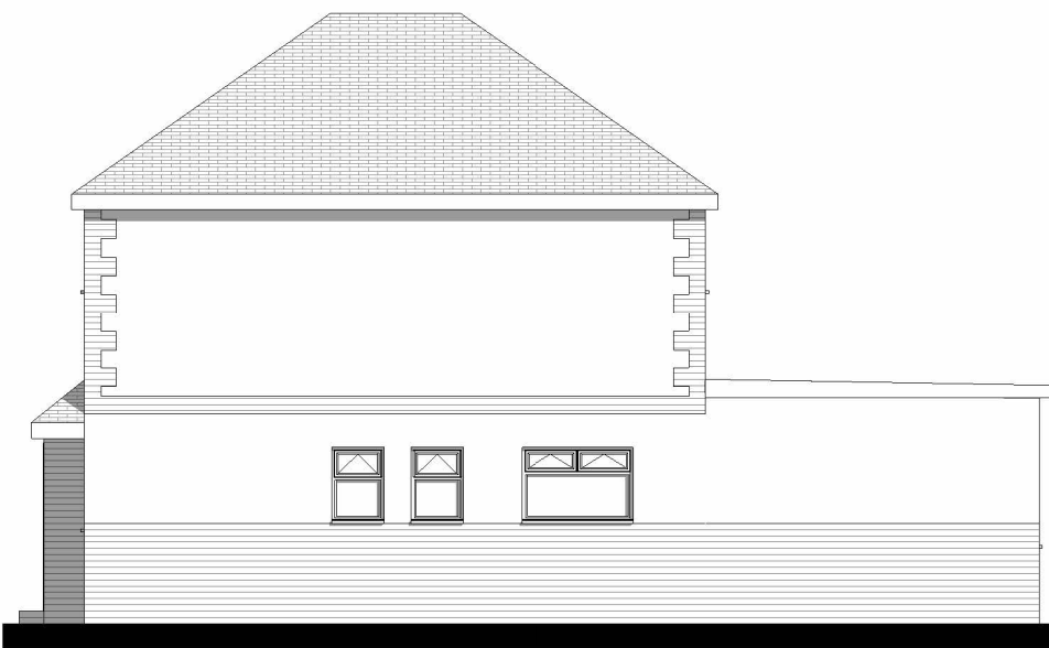
6 Side Elevation 1 : 100
