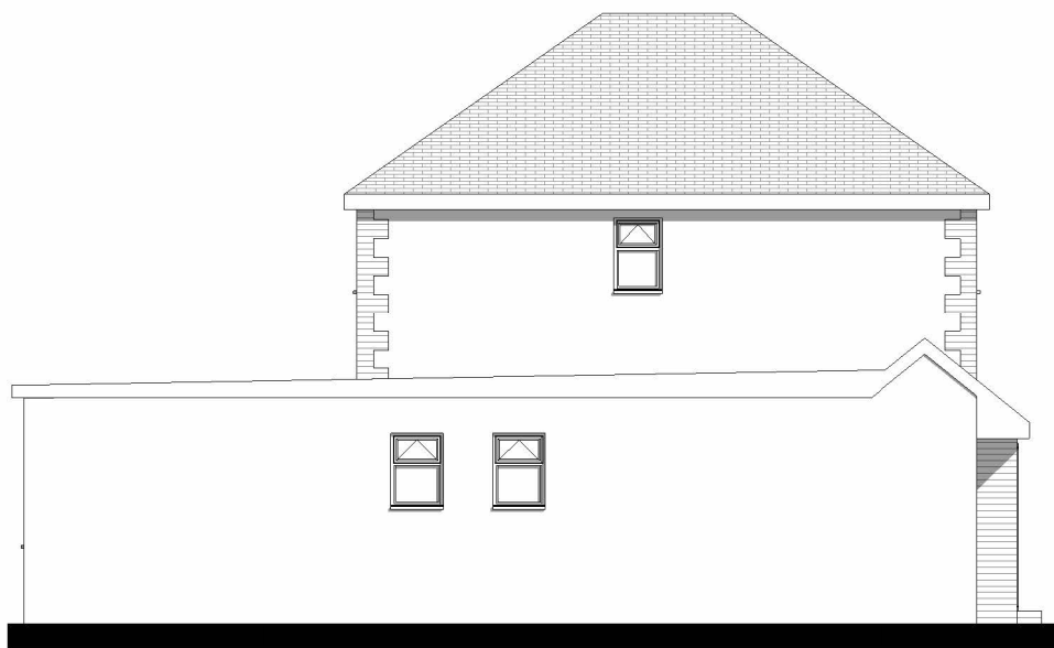
5 Side Elevation 1 : 100
