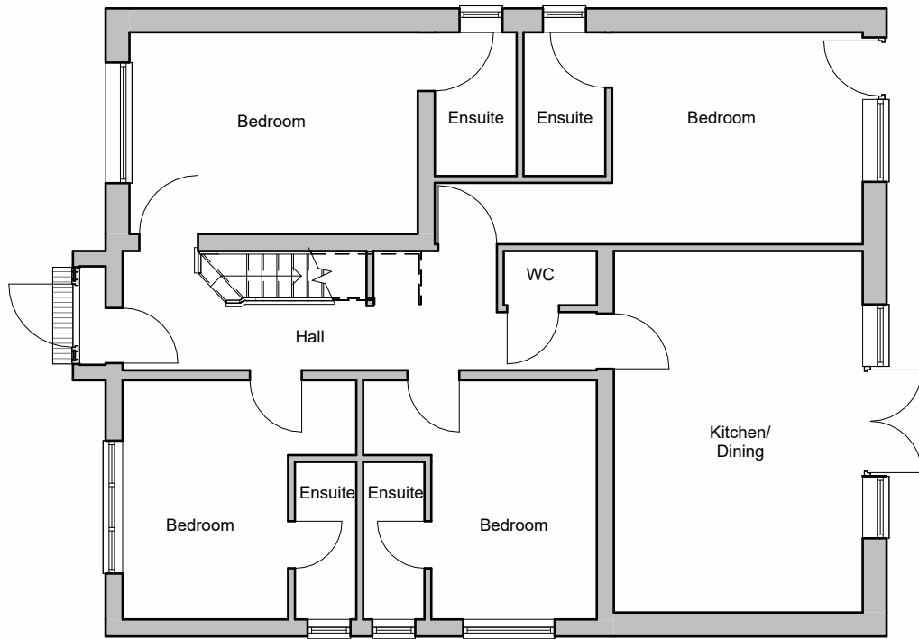
2 Ground Floor 1 : 100
