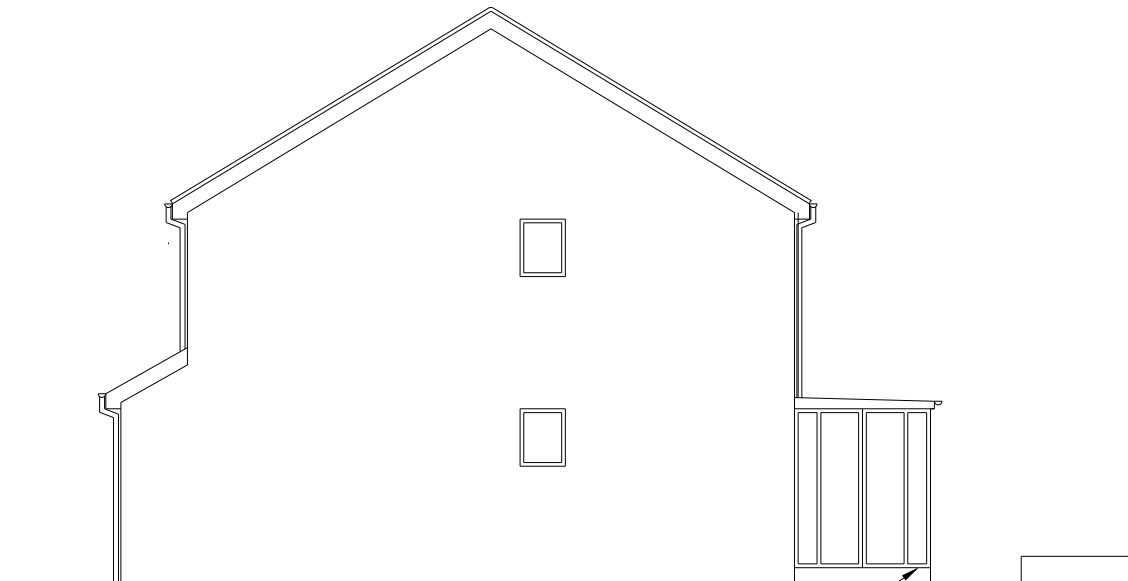
RIGHTSIDE ELEVATION EXISTING
