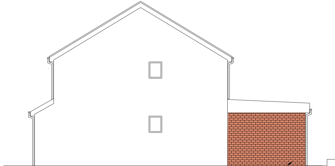
RIGHTSIDE ELEVATION PROPOSED
