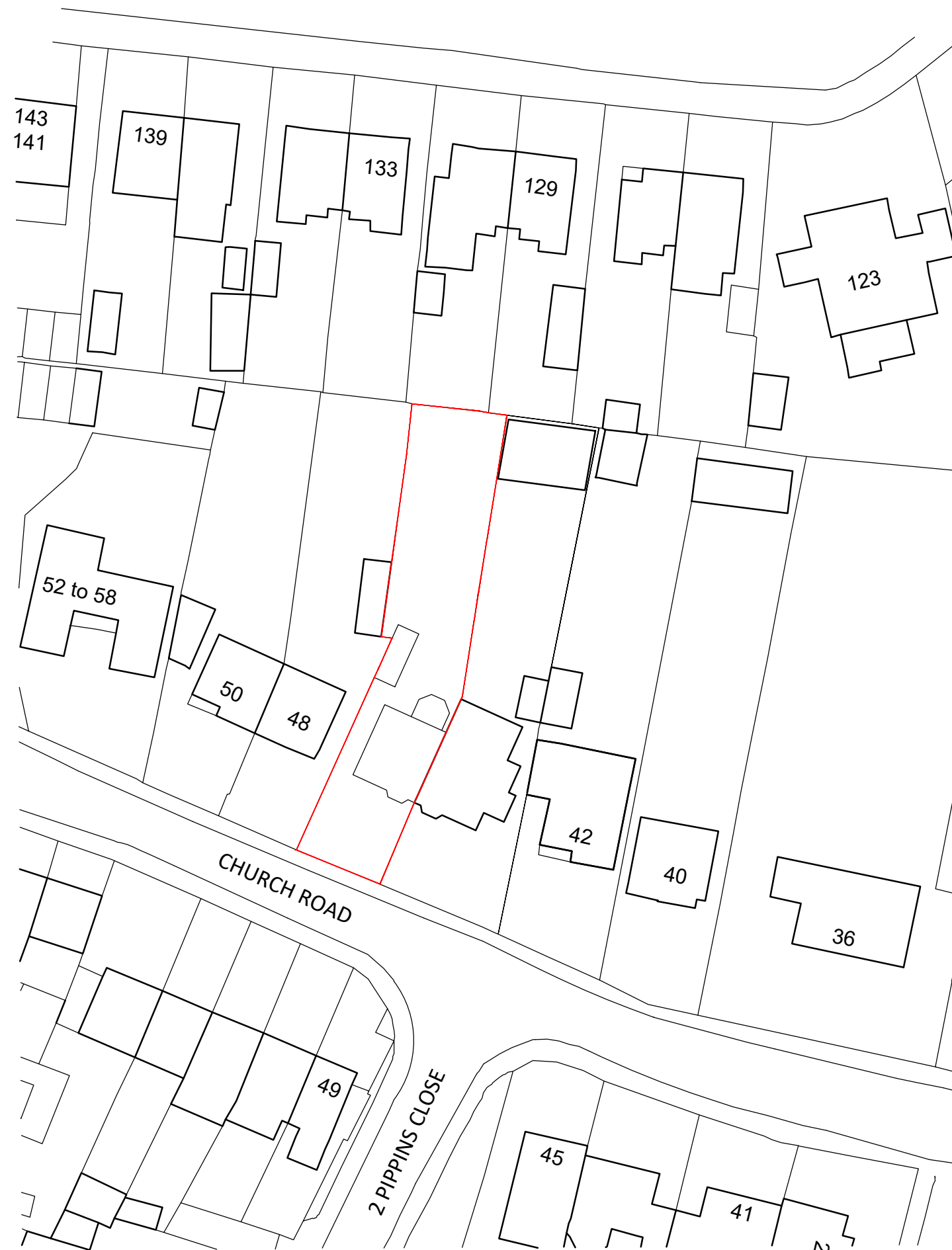
BLOCK PLAN @1:500
