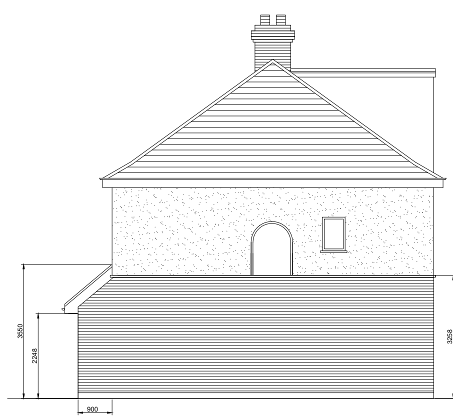
2 SIDE ELEVATION - PROPOSED Scale: 1:100
