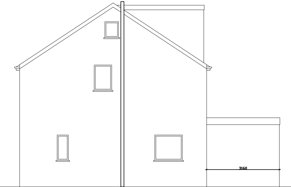
Side Elevation (No. 27)
