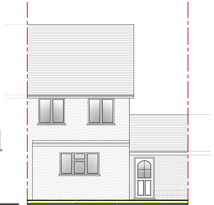
6 Existing Rear Elevation
