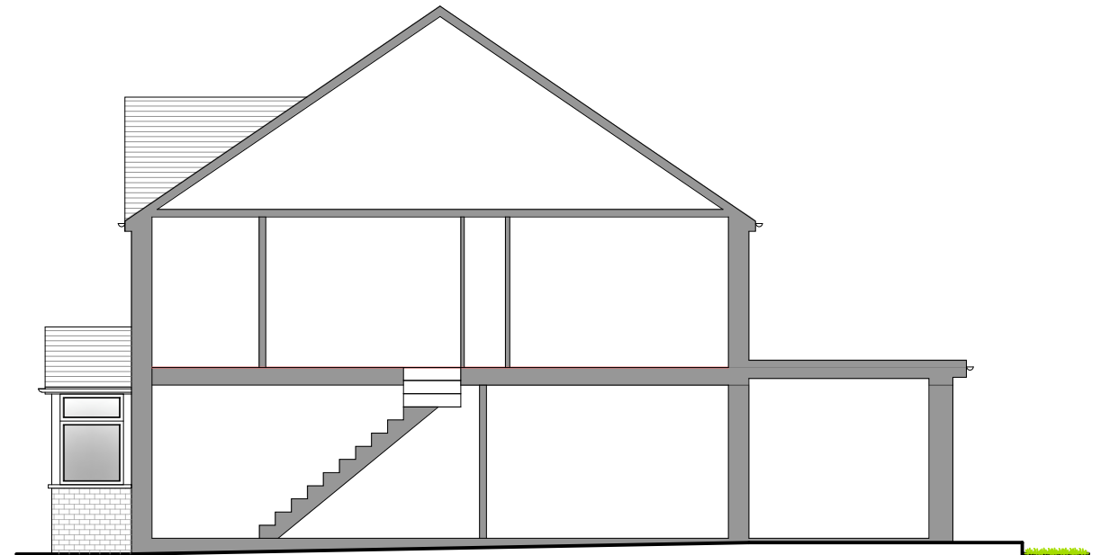
8 Existing Side Section
