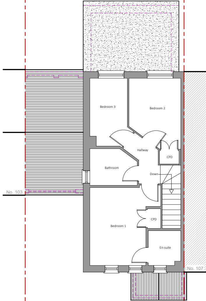
2 Existing First Floor Plan
