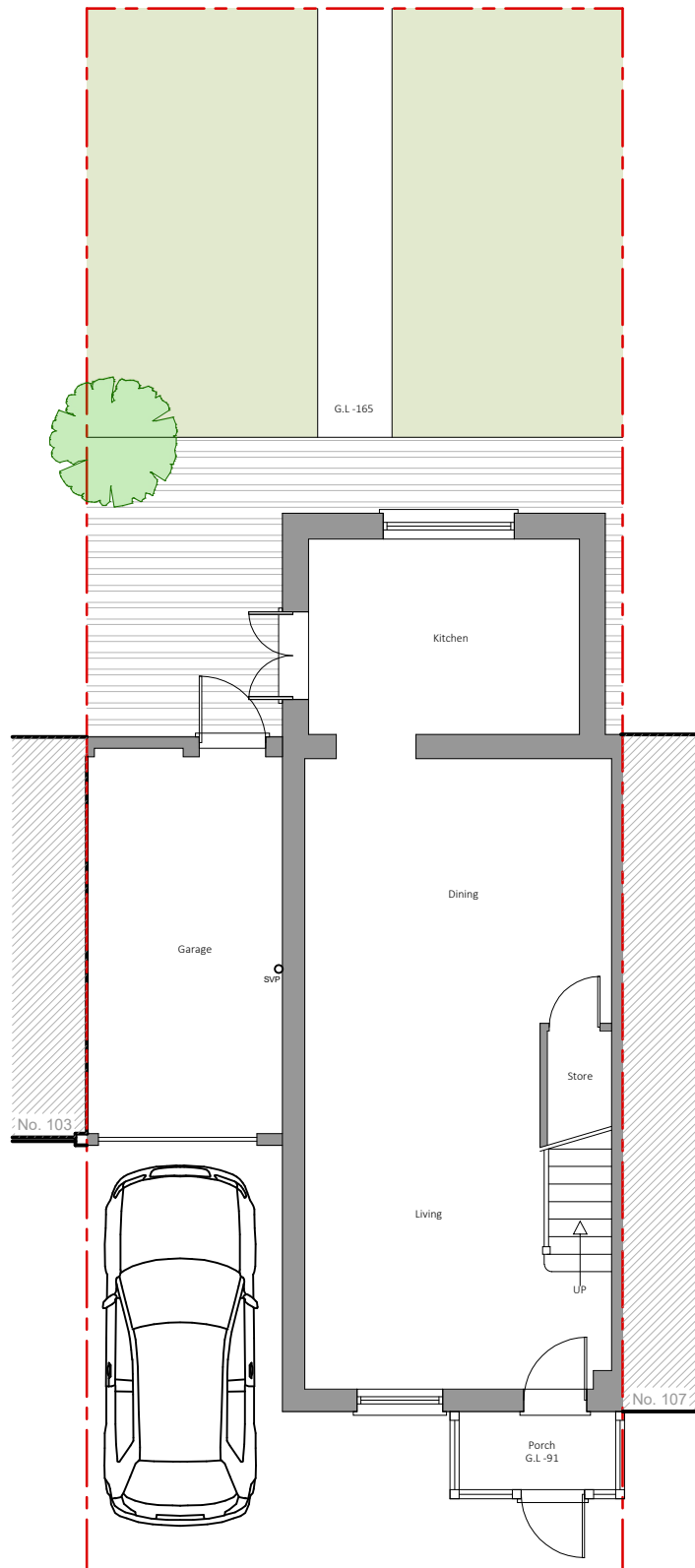
1 Existing Ground Floor Plan
