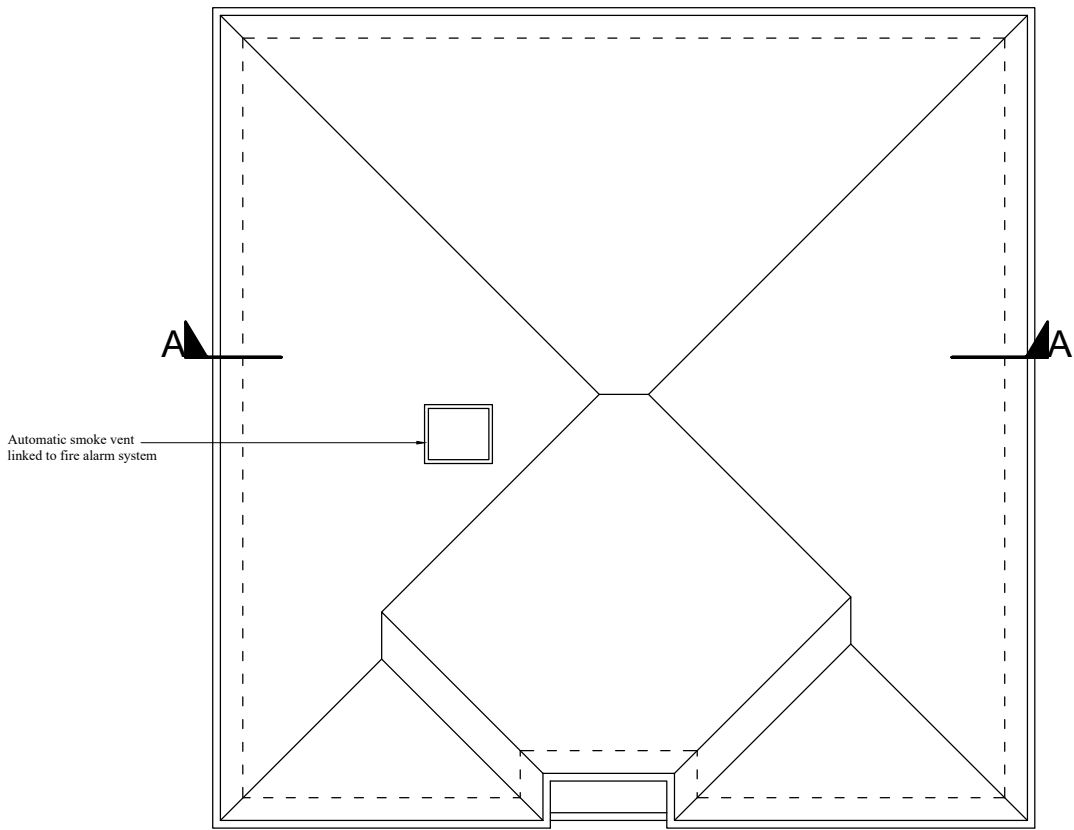
roof plan
