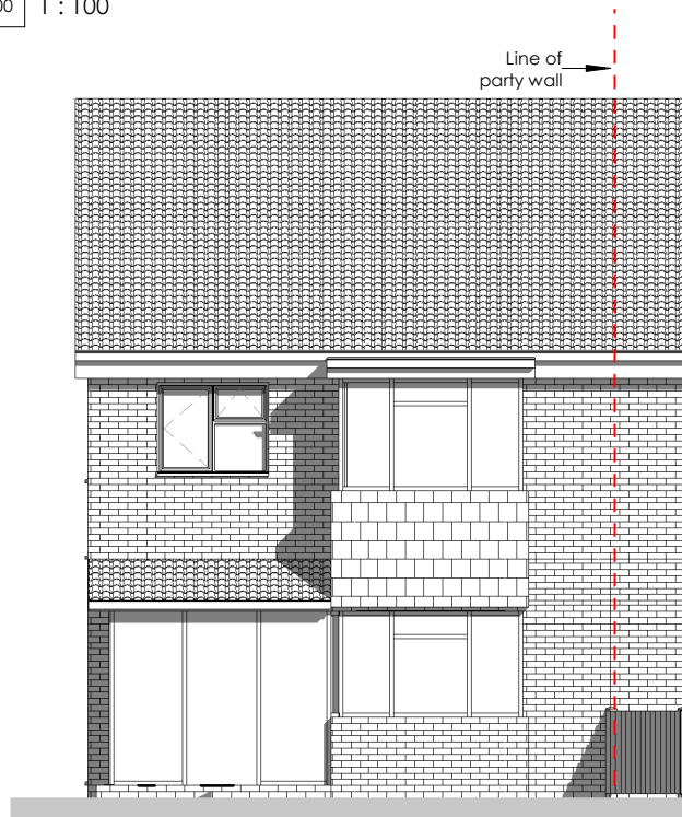
3 Existing Front Elevation 2326-A-200 1 : 100
