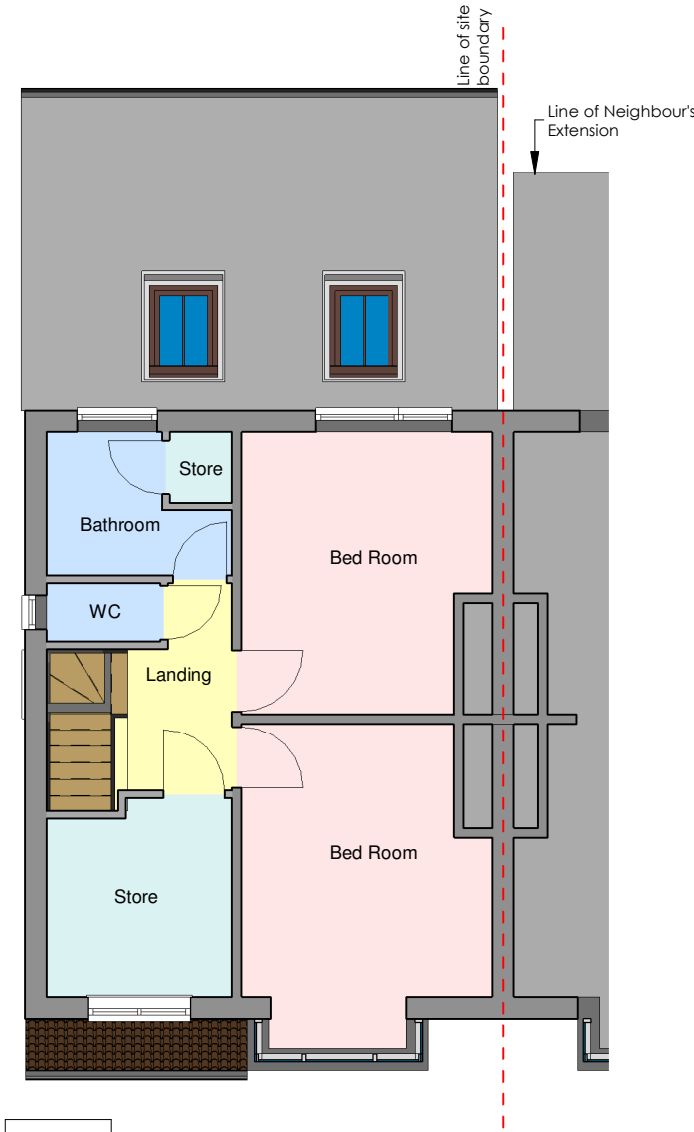
2 Proposed First Floor 2326-A-301 1 : 100
