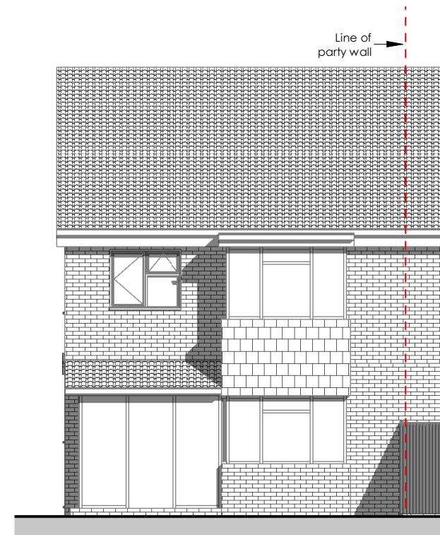
3 Front Elevation (Proposed) 2326-A-301 1 : 100
