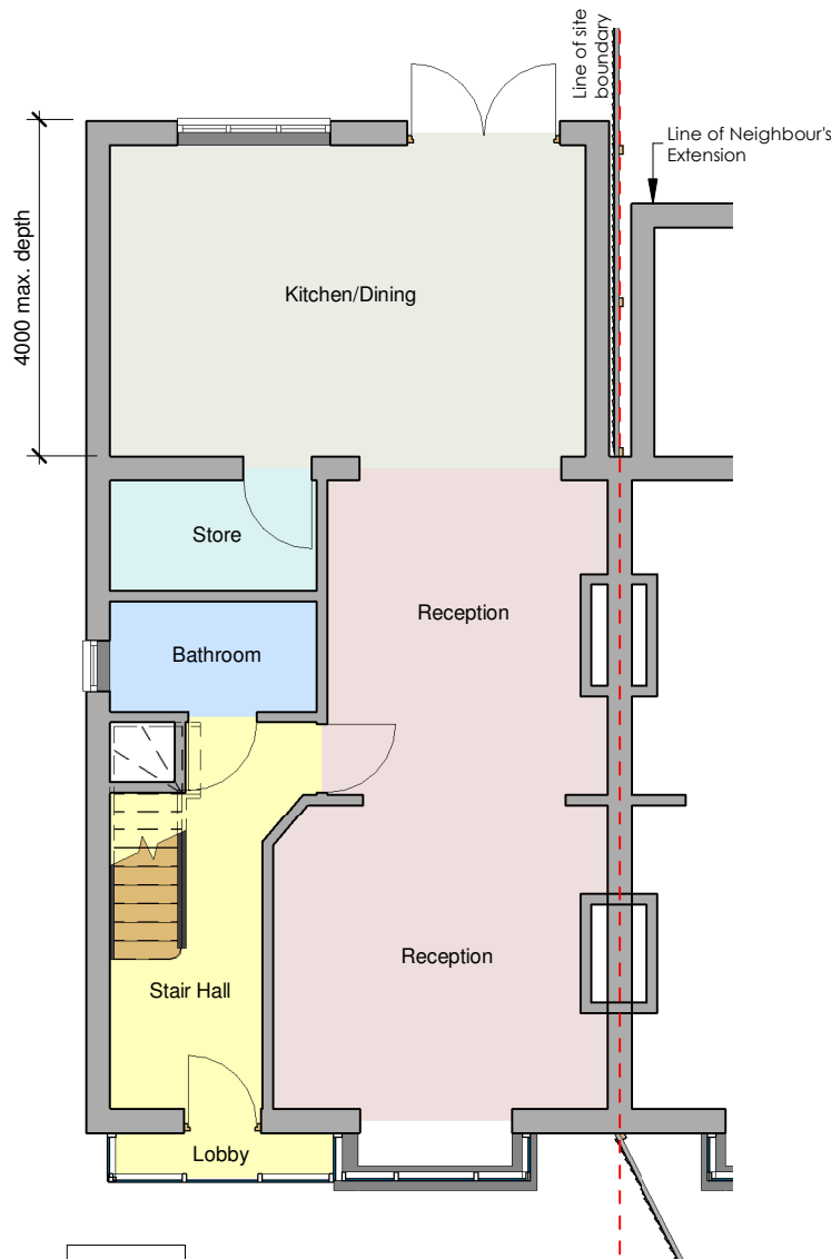
1 Proposed Ground Floor 2326-A-301 1 : 100
