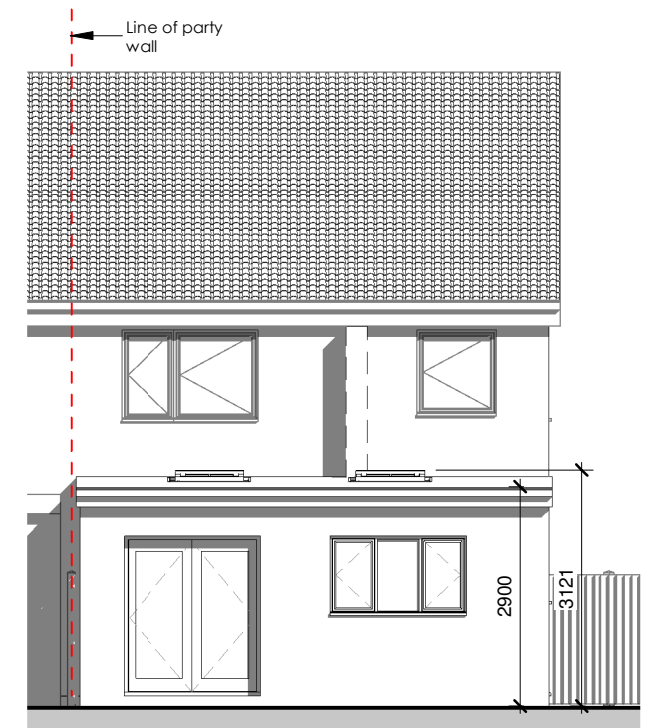
4 Rear Elevation (Proposed) 2326-A-301 1 : 100
