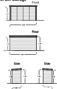
Elevation of Bin Storage
