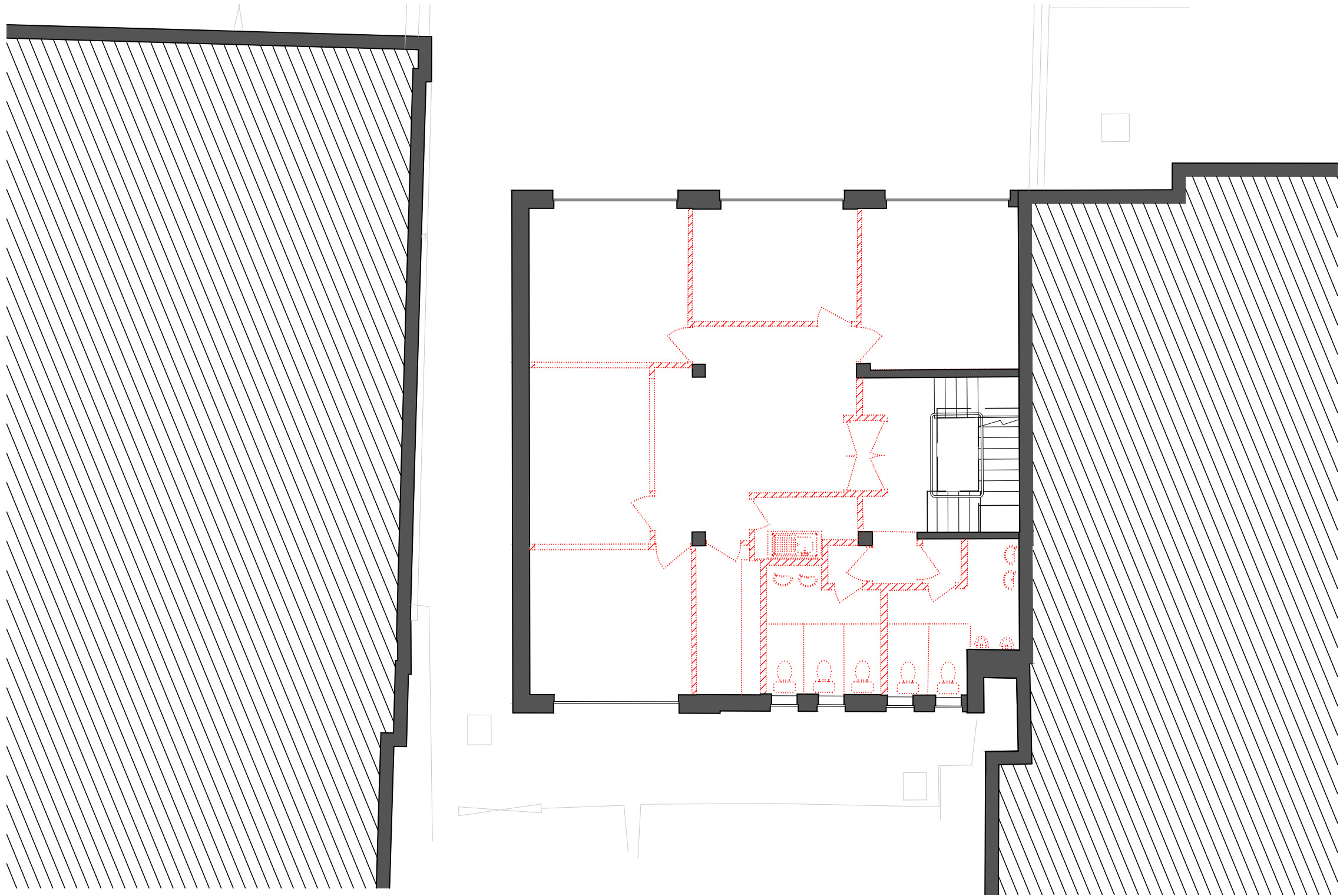
Demolition: First Floor Plan
