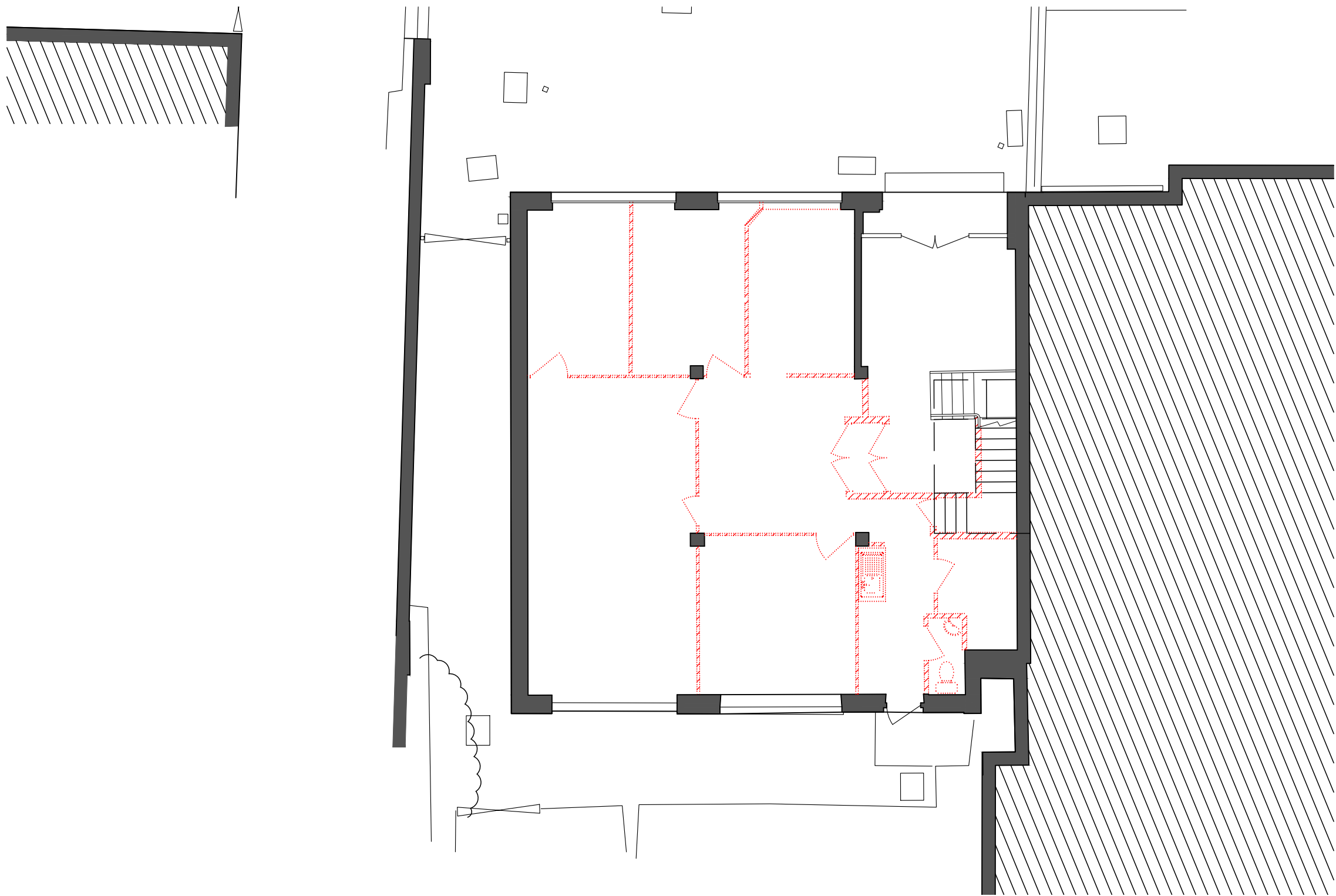
Demolition: Ground Floor Plan
