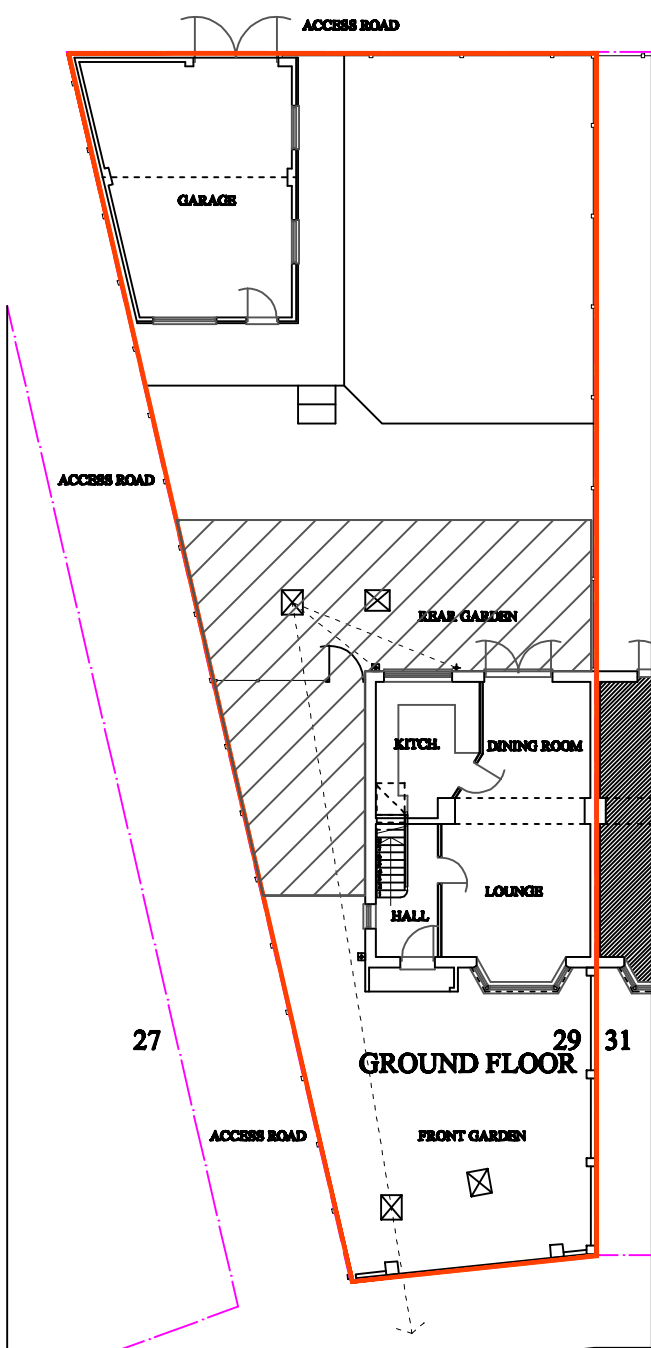
PLOT PLAN 1:200
