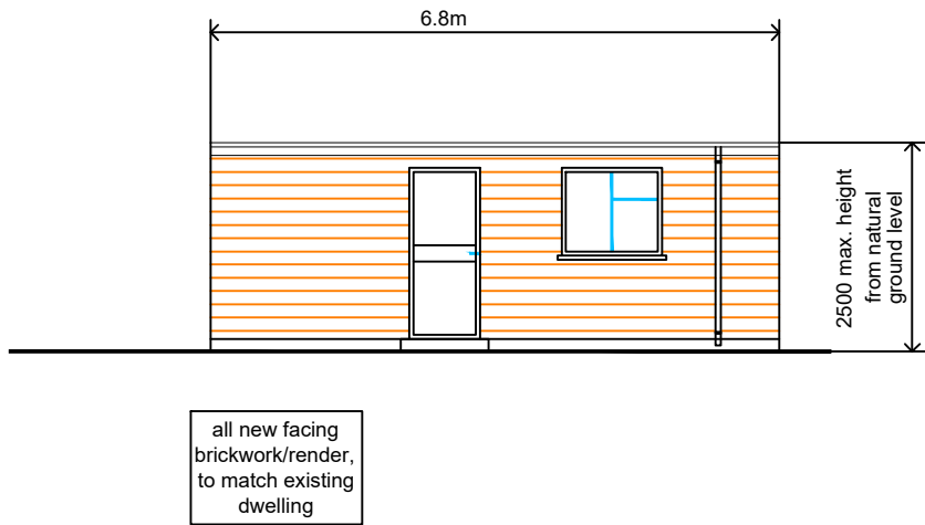
Front Elevation - Out Building
