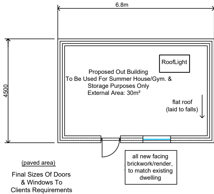
Proposed Out Building Ground Floor Layout
