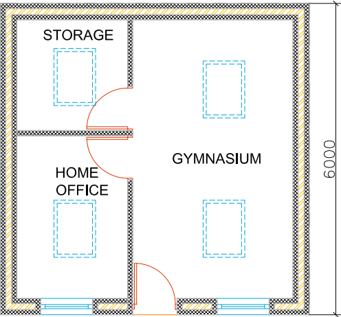
PROPOSED OUT-BUILDING
