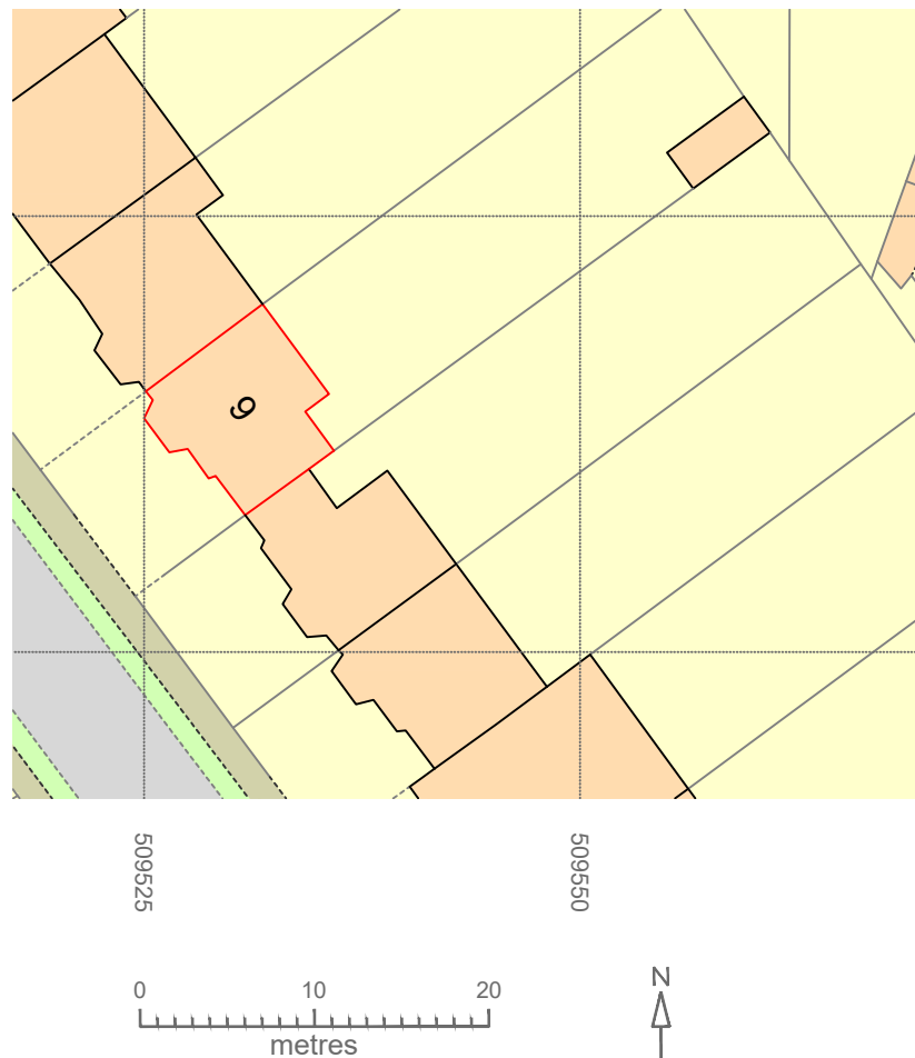
Block plan (1:500)
