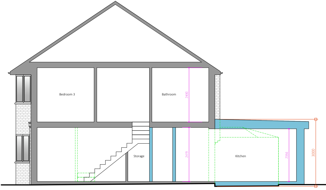
8 Proposed Side Section
