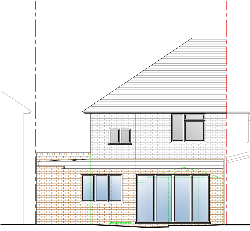
5 Proposed Rear Elevation
