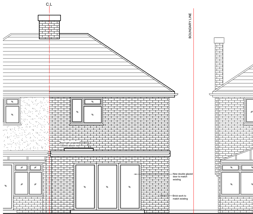
04 - REAR ELEVATION
