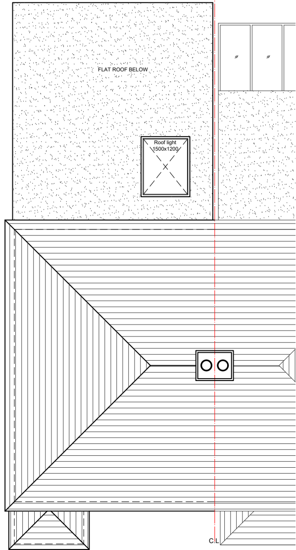
03 - ROOF PLAN
