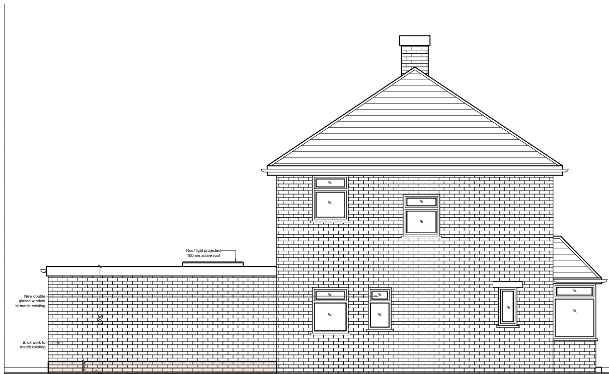
05 - SIDE ELEVATION
