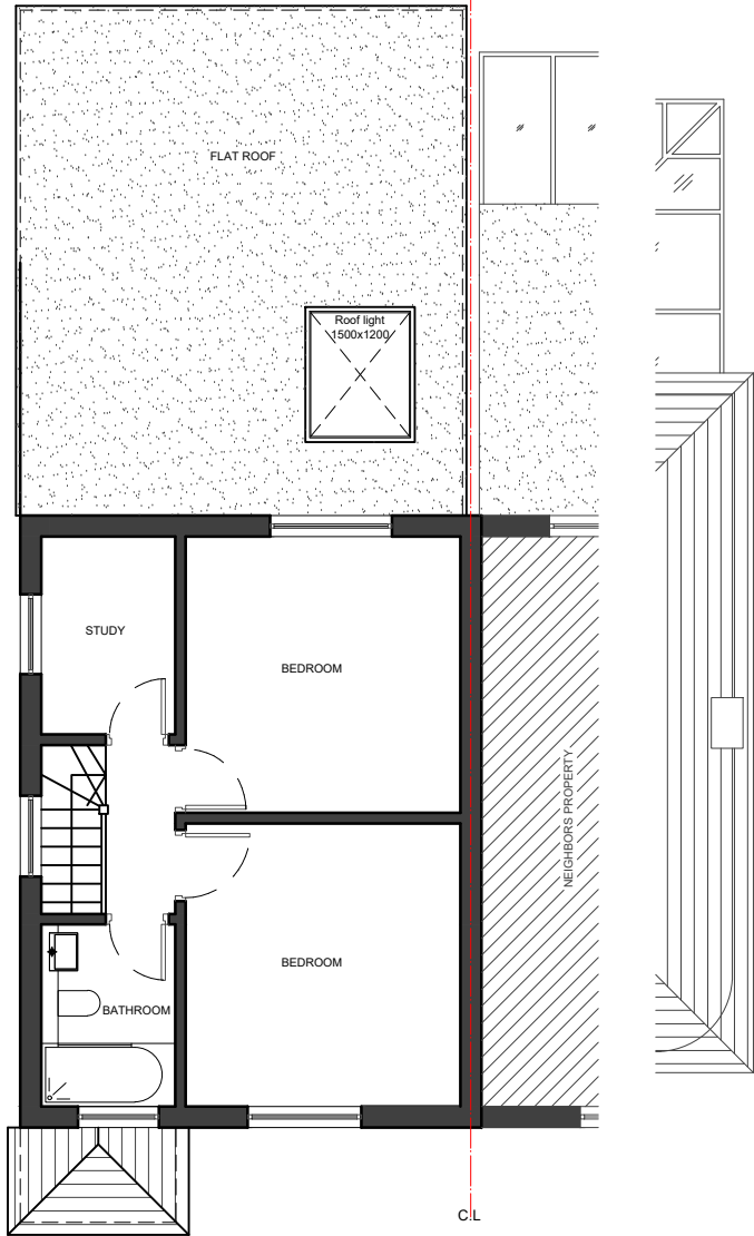
02 - FIRST FLOOR PLAN
