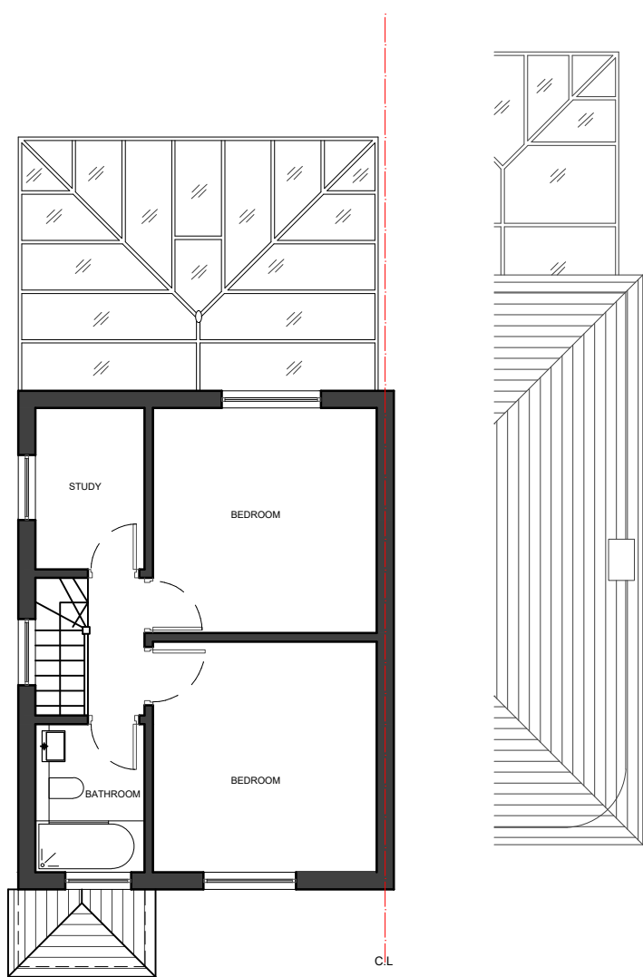
05 - FIRST FLOOR PLAN
