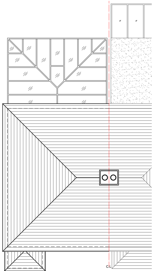
06 - ROOF PLAN
