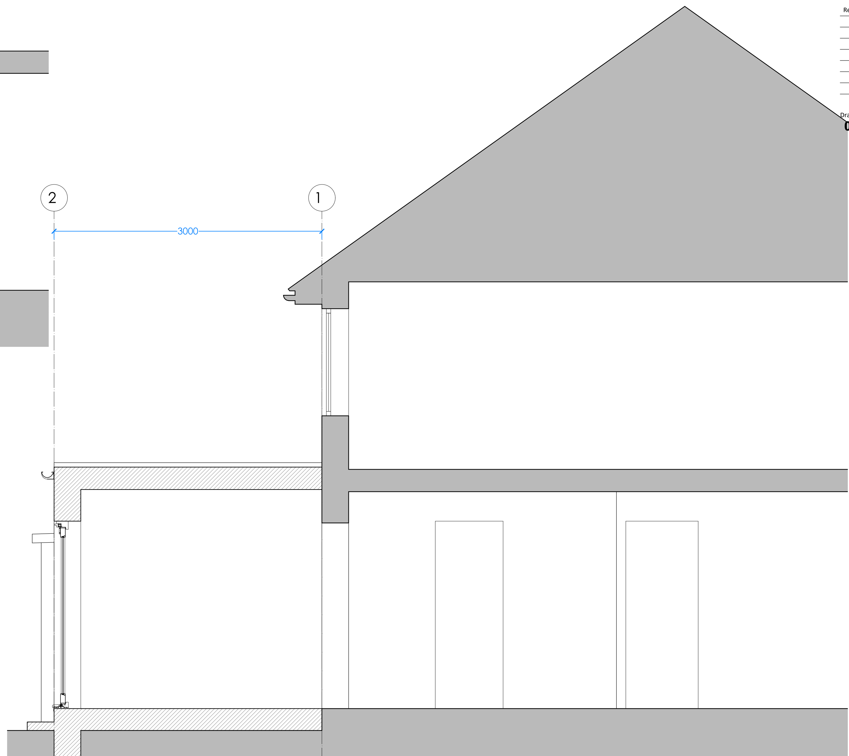
2. PROPOSED SECTION AA 1:25@A1/ 1:50@A3
