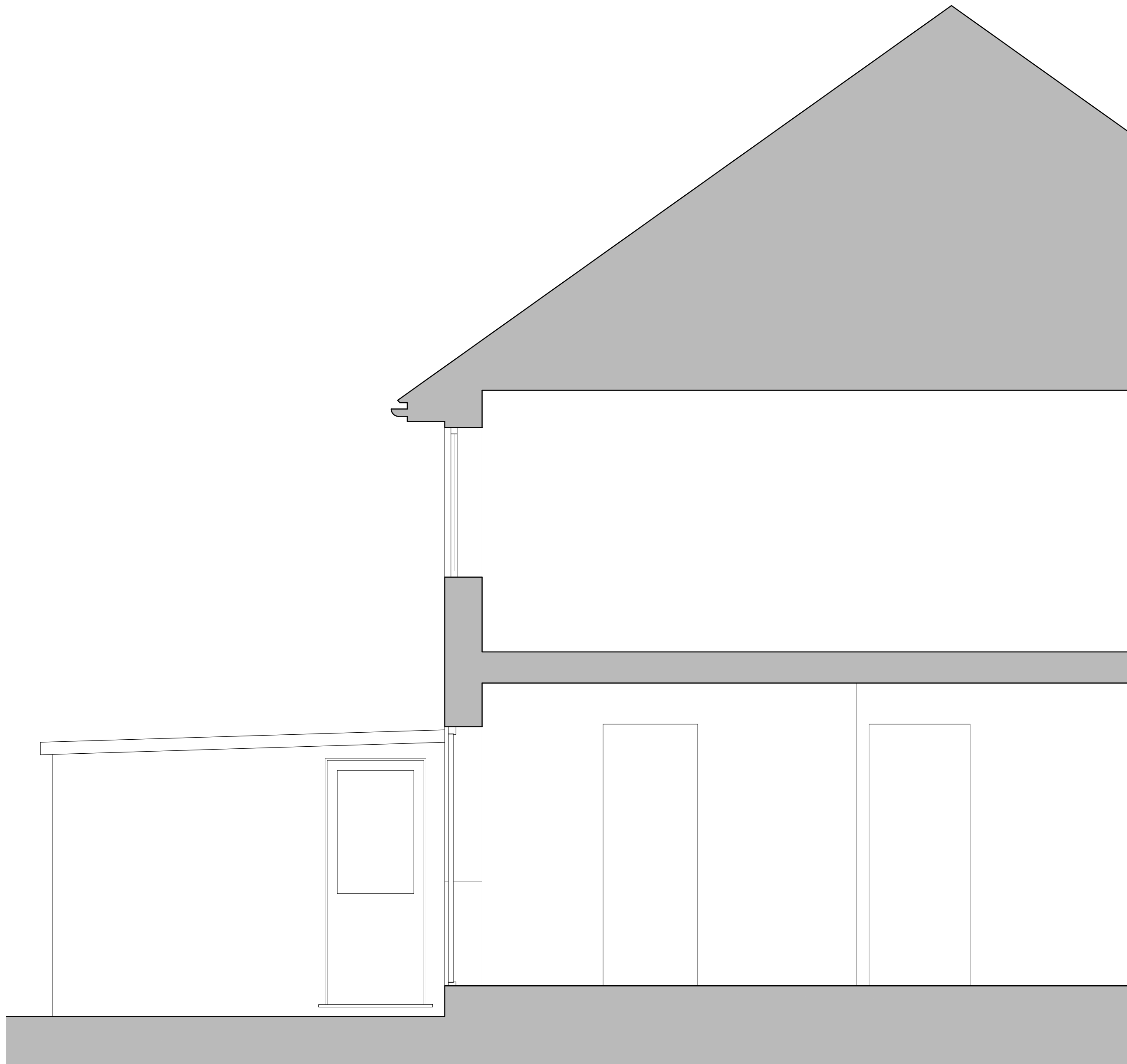
1. EXISTING SECTION AA 1:25@A1/ 1:50@A3
