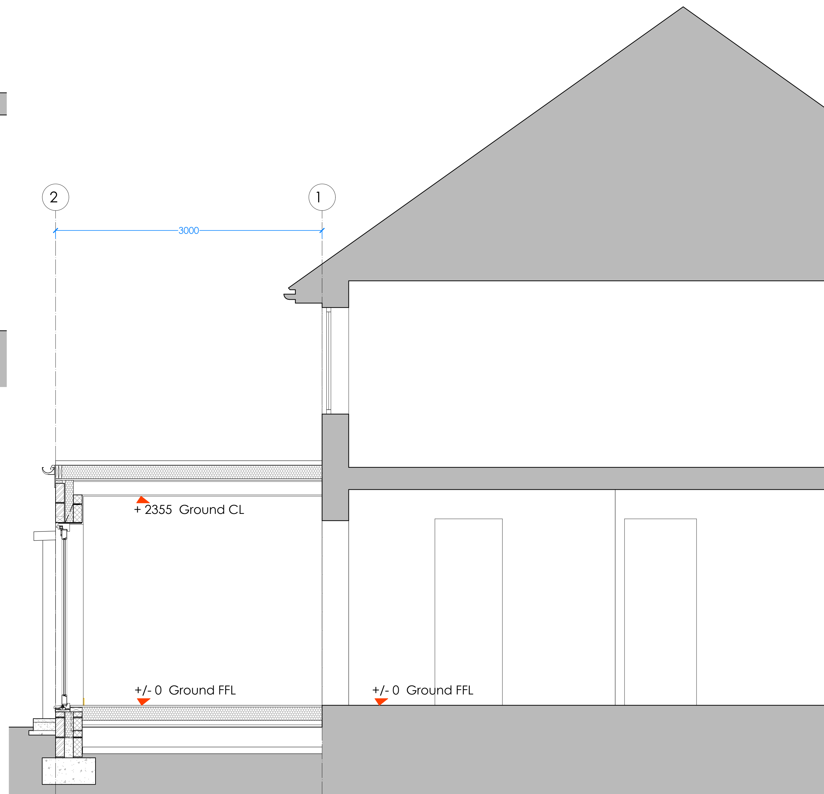
2. PROPOSED SECTION AA 1:25@A1/ 1:50@A3
