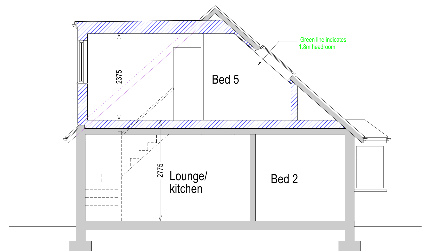
Section (1:50)
