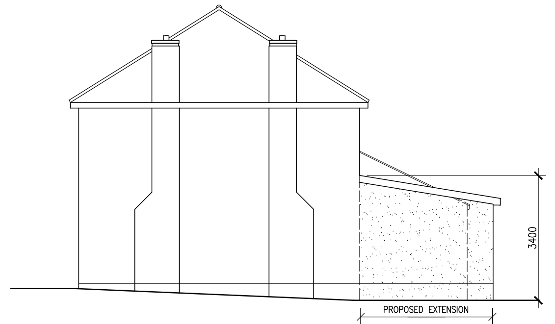
SIDE ELEVATION
