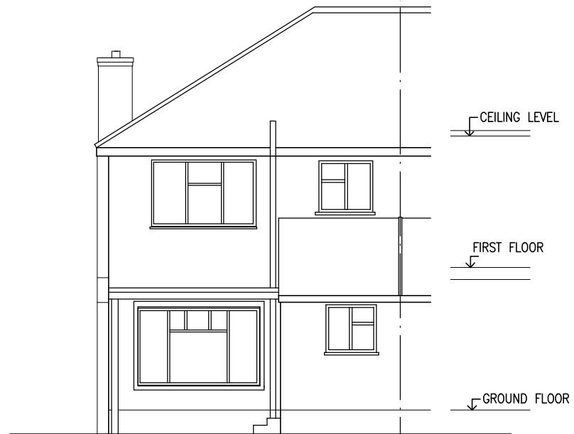
REAR ELEVATION
