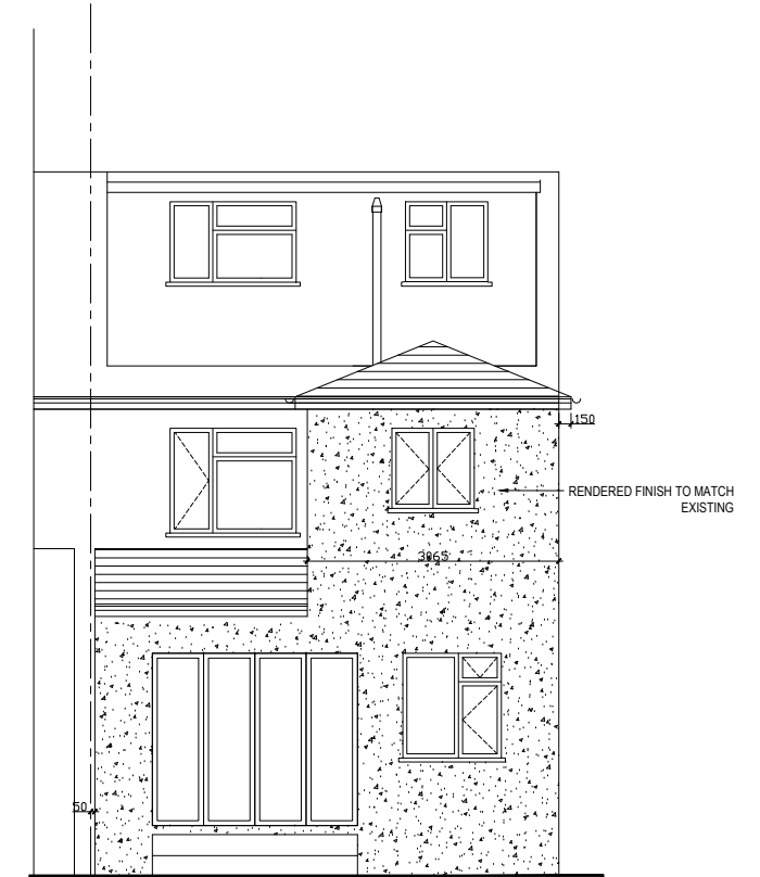
Rear Elevation
