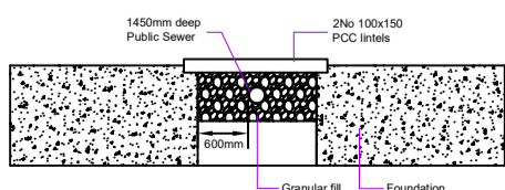
SEWER BRIDGING SECTION DETAIL
