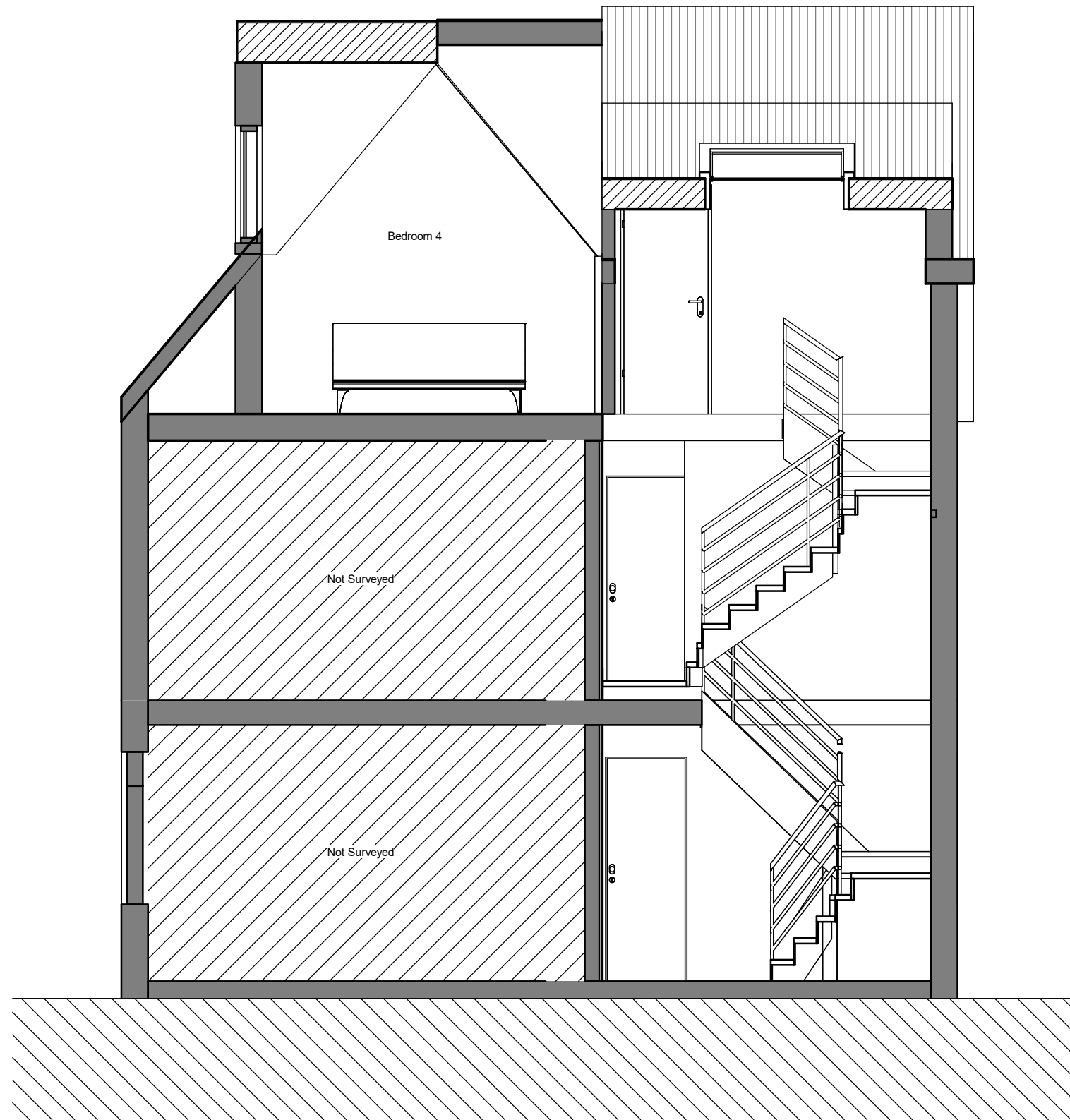
Proposed - Section BB 1 : 50
