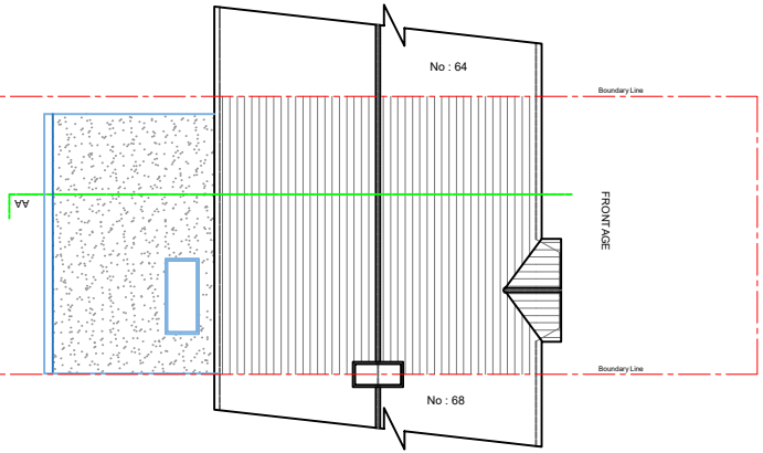
PROPOSED ROOF/BLOCK PLAN SCALE : 1/200
