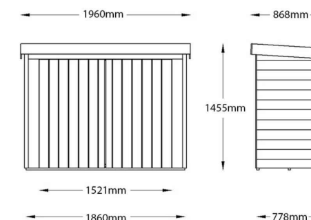
DETAILS OF CYCLE SHED
