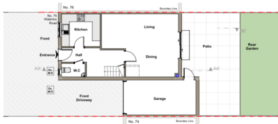
Existing Ground Floor Plan 1:100
