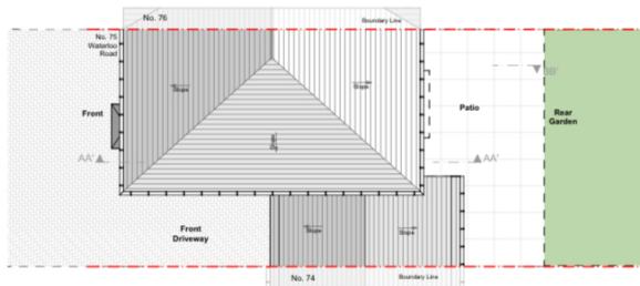
Existing Roof Plan 1:100
