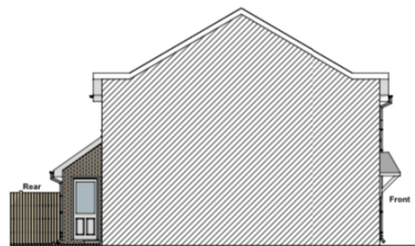
Existing Flank Elevation 1:100
