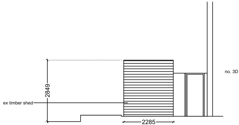
03. South Elevation Pre-existing 1 : 100
