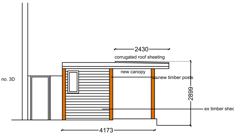
04. North Elevation Existing 1 : 100
