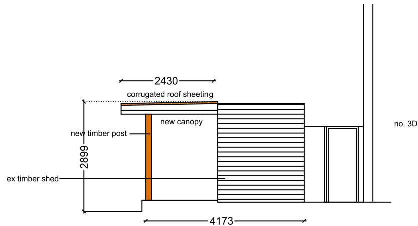
03. South Elevation Existing 1 : 100
