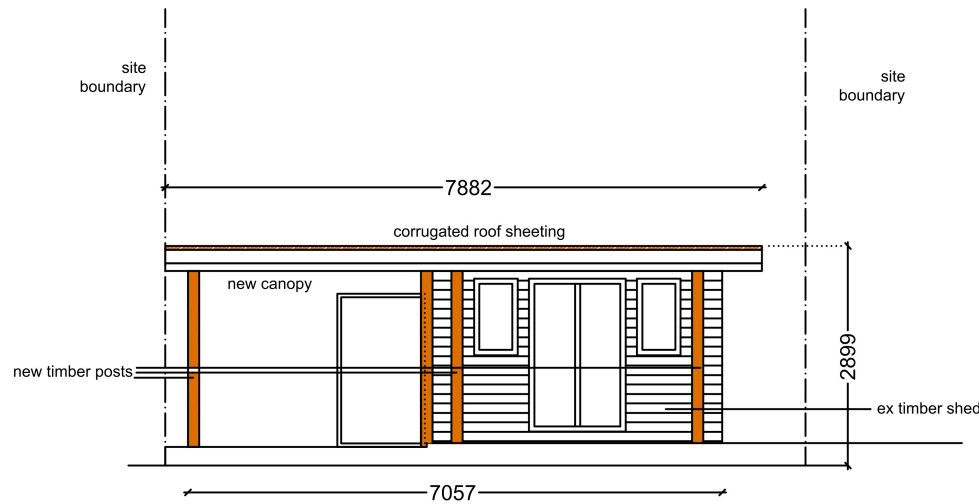
01. East Elevation Existing 1 : 100
