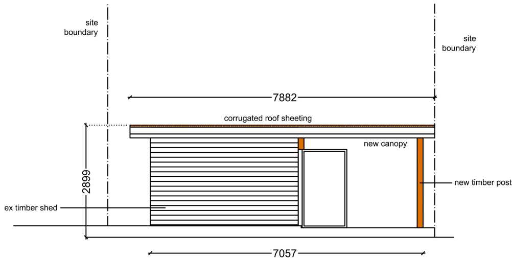
02. West Elevation Existing 1 : 100
