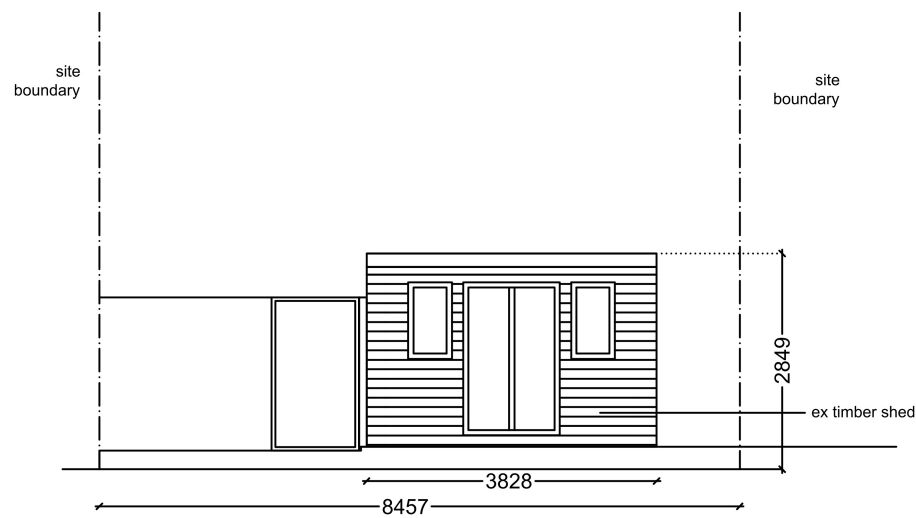
01. East Elevation Pre-existing 1 : 100
