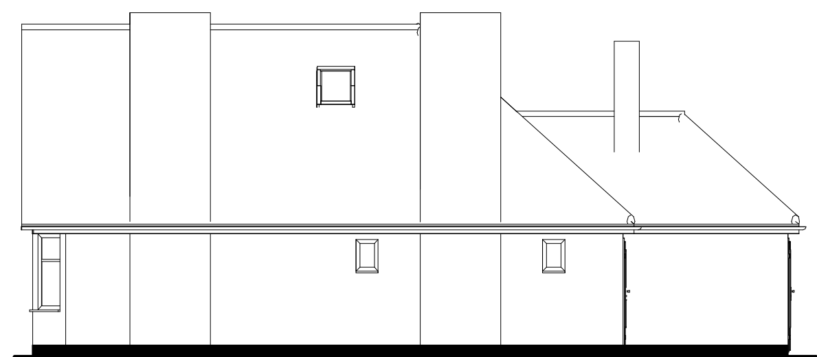
EXISTING RIGHT HAND SIDE ELEVATION
