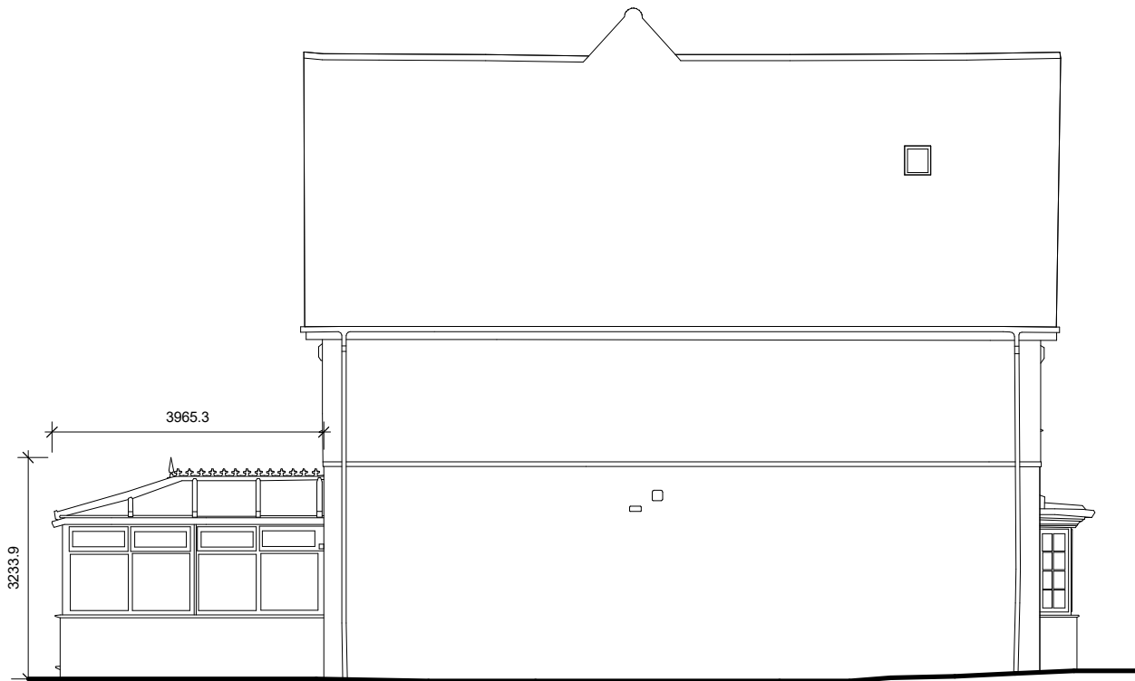
2 EXISTING SOUTH SIDE ELEVATION 1 : 100
