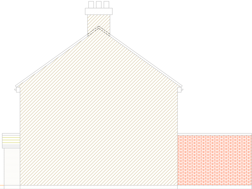
PROPOSED SIDE ELEVATION-1
