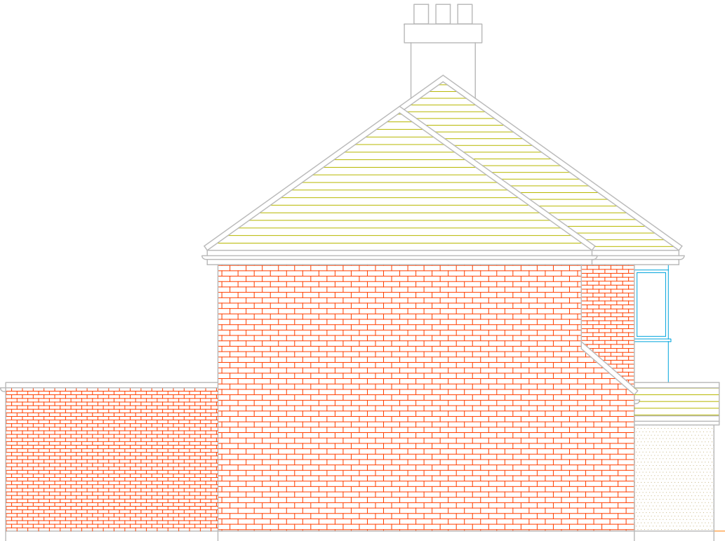
PROPOSED SIDE ELEVATION-2
