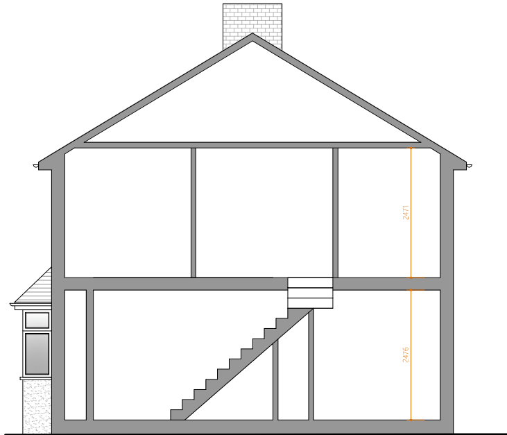
8 Existing Side Section
