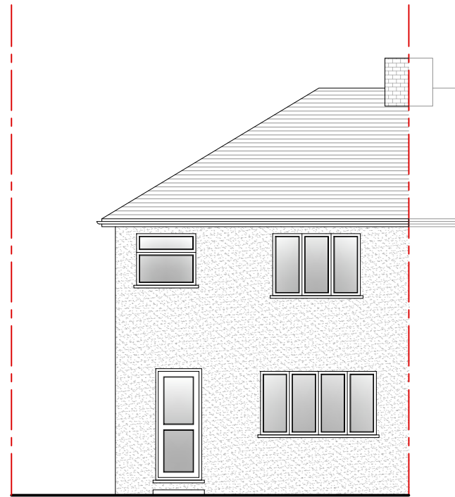
6 Existing Rear Elevation
