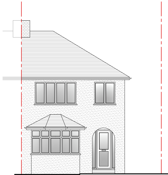
4 Existing Front Elevation
