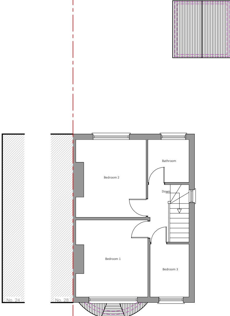
2 Existing First Floor Plan
