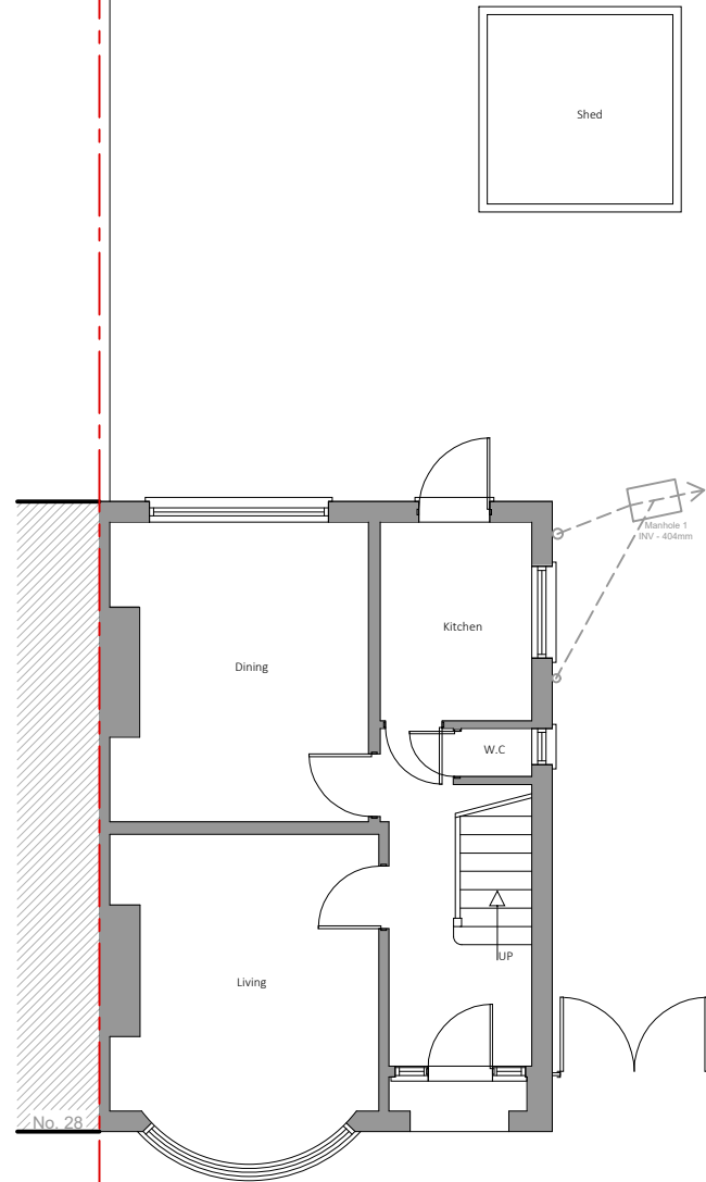
1 Existing Ground Floor Plan
