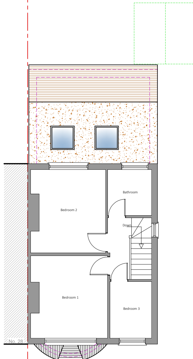
2 Proposed First Floor Plan
