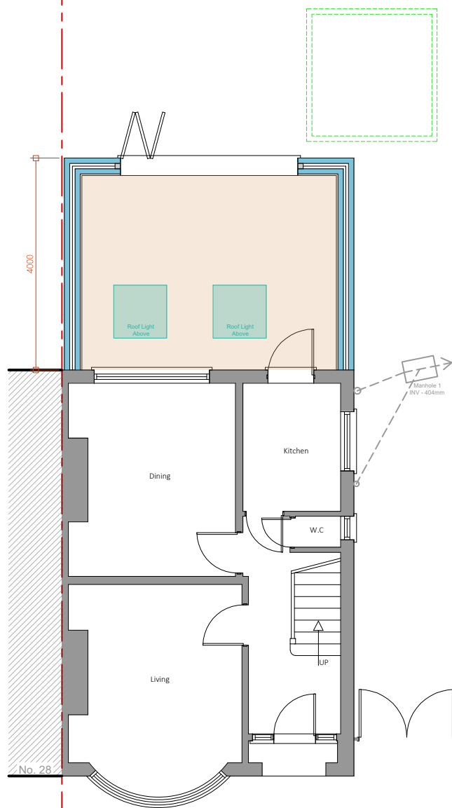
1 Proposed Ground Floor Plan
