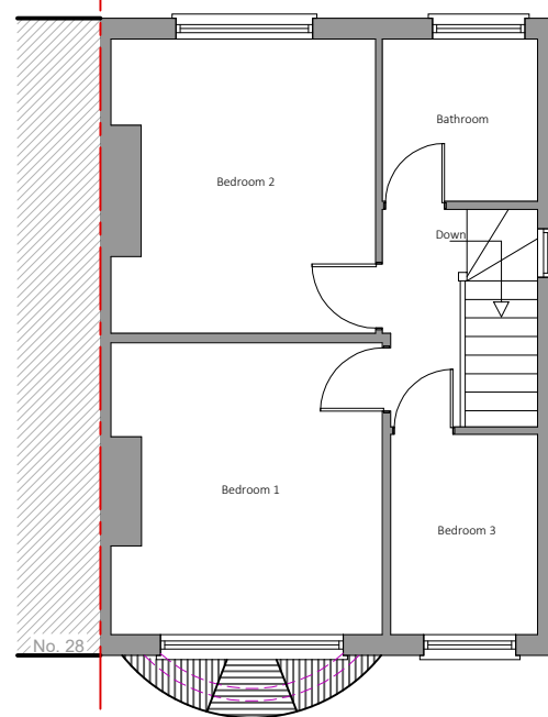
2 Existing First Floor Plan
