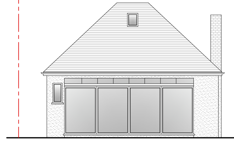
5 Existing Rear Elevation
