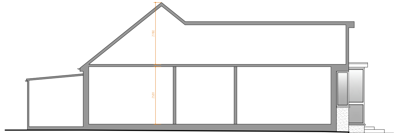
7 Existing Side Section
