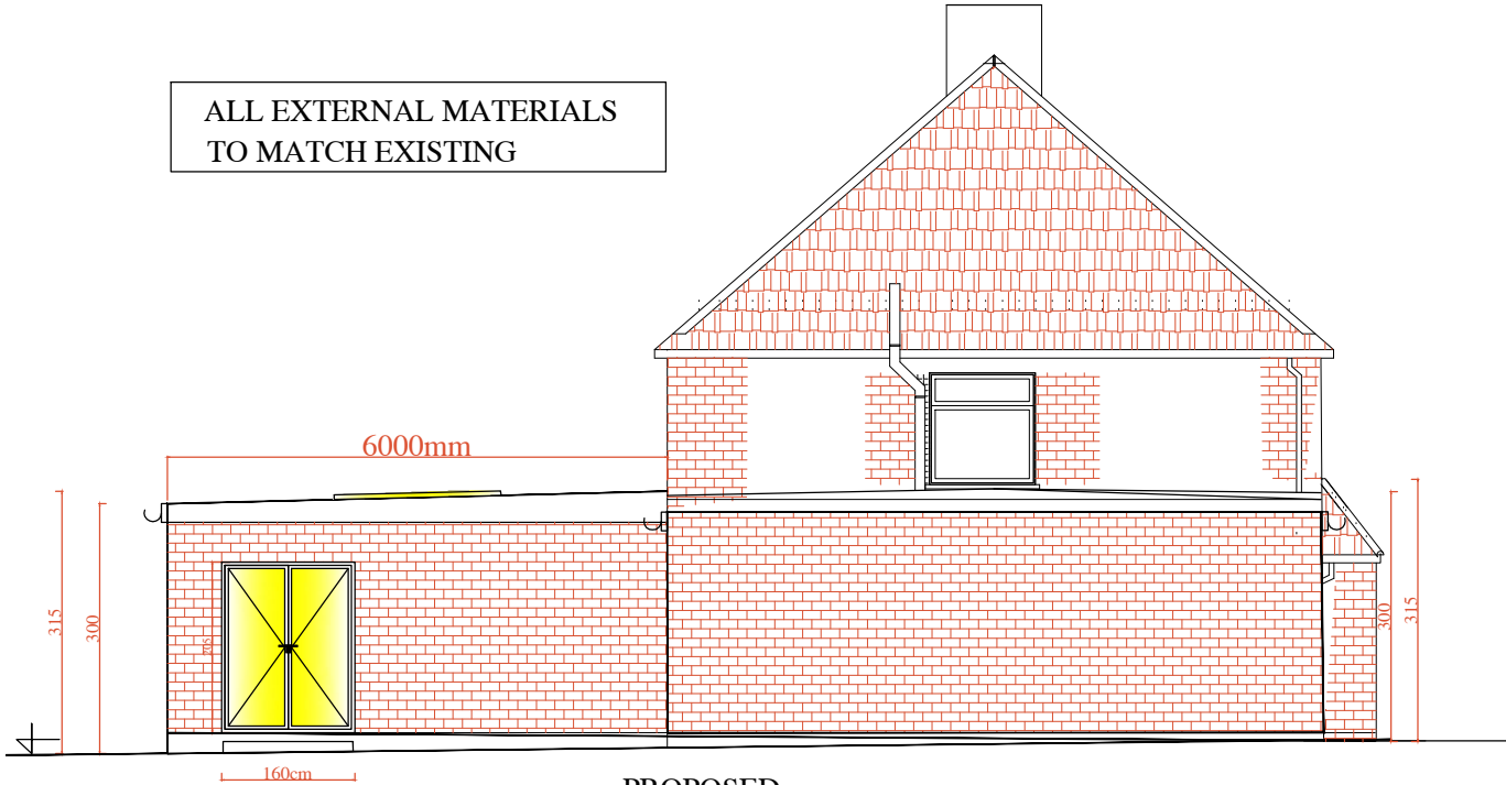
PROPOSED DETACHED SIDE ELEVATION NORTH WEST ELEVATION
