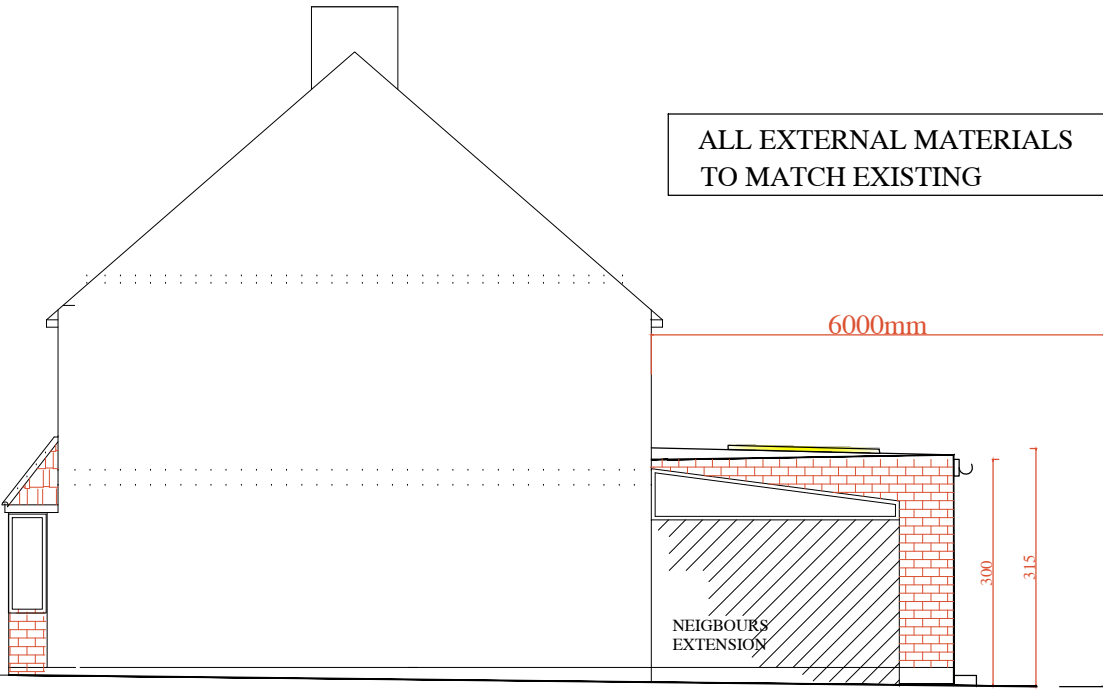
PROPOSED SIDE ELEVATION SOUTH EAST ELEVATION
