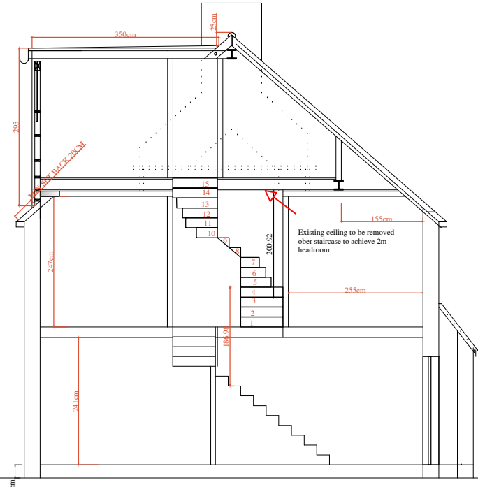
PROPOSED SECTION A-A
