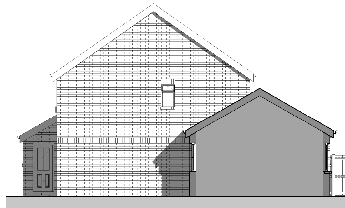
4 Proposed Side Elevation (South) 2308-A-200 1 : 100
