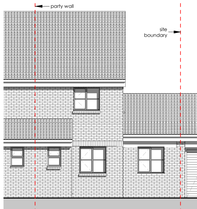
3 Proposed Front Elevation 2308-A-200 1 : 100
