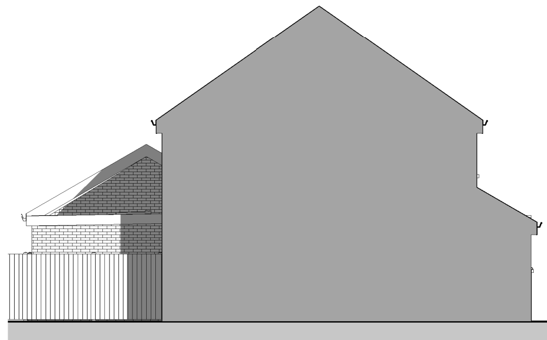
6 Proposed Side Elevation (North) 2308-A-200 1 : 100
