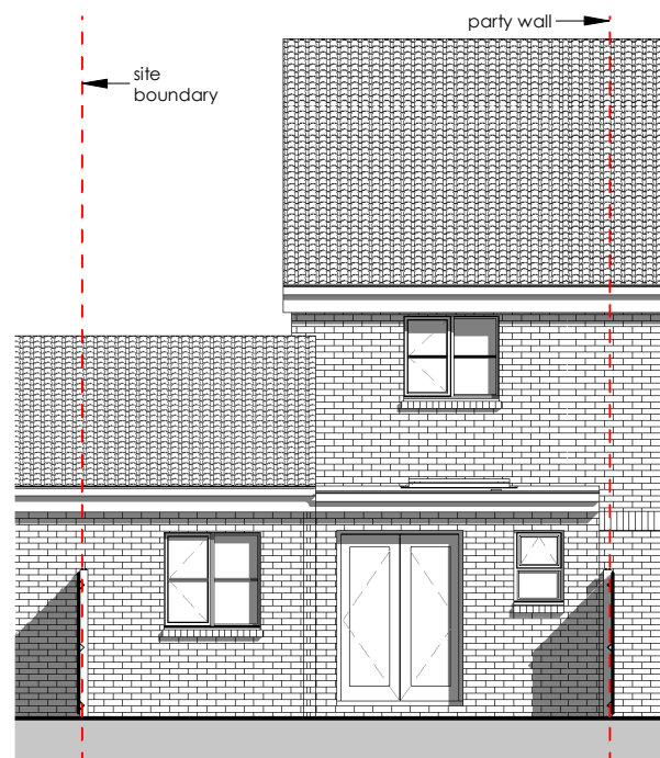
5 Proposed Rear Elevation 2308-A-200 1 : 100
