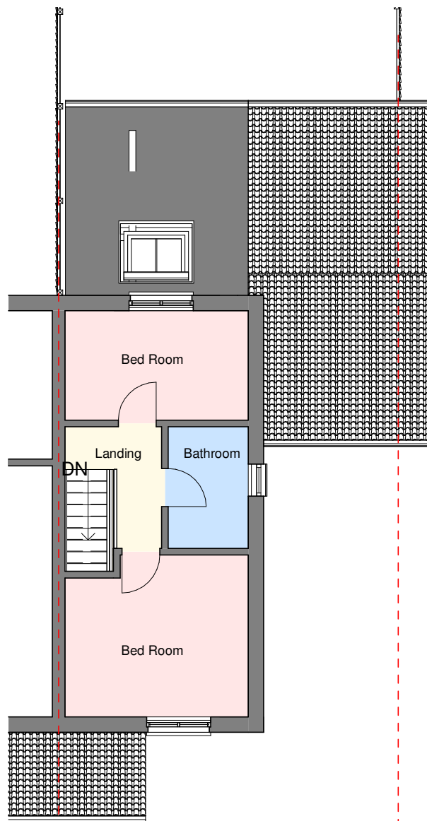
2 Proposed First Floor Plan 2308-A-200 1 : 100
