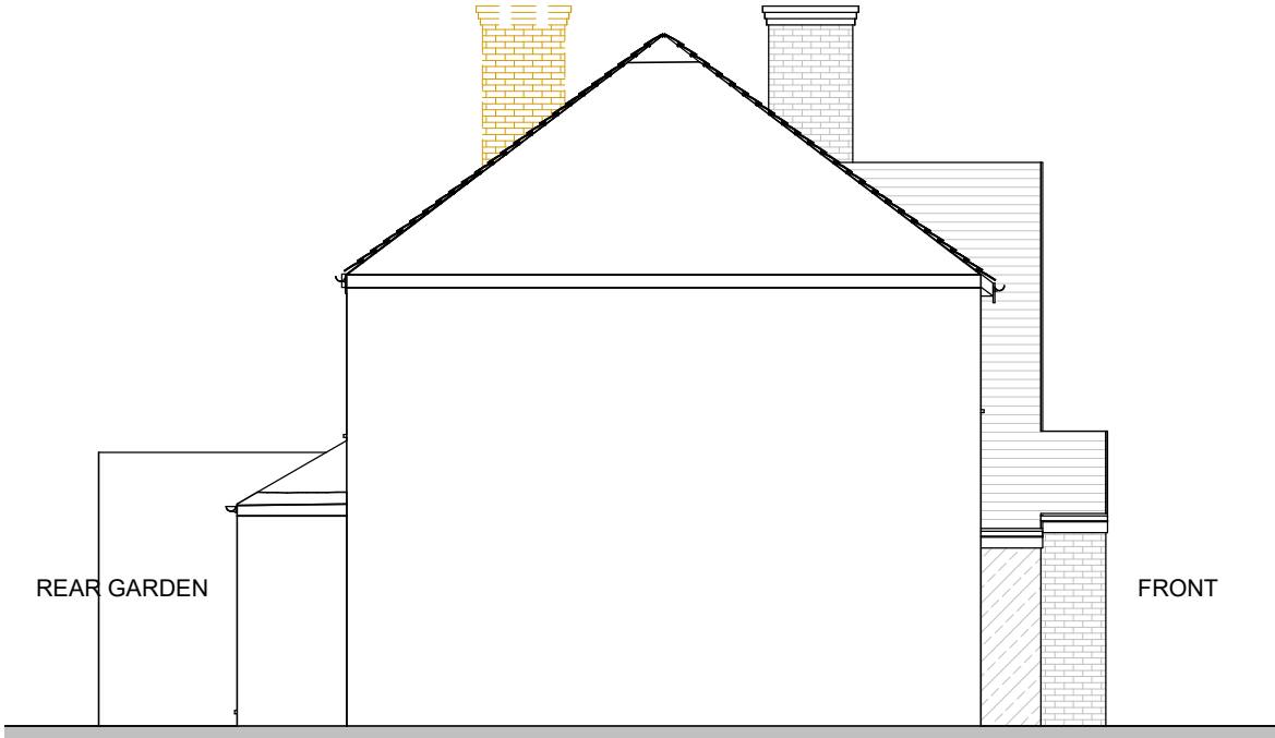
PP-EXISTING LEFT SIDE ELEVATION 1 : 100
