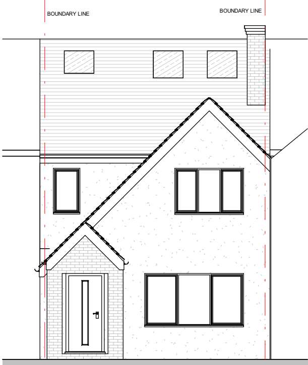
PP-EXISTING FRONT ELEVATION 1 : 100
