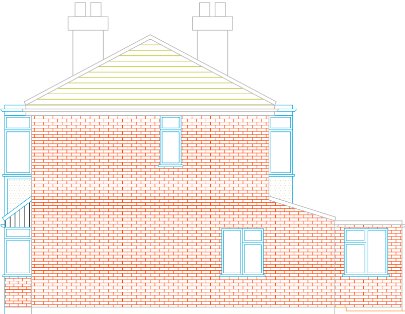
EXISTING SIDE ELEVATION-1
