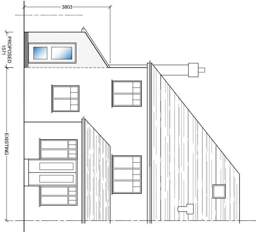
NORTH ELEVATION
