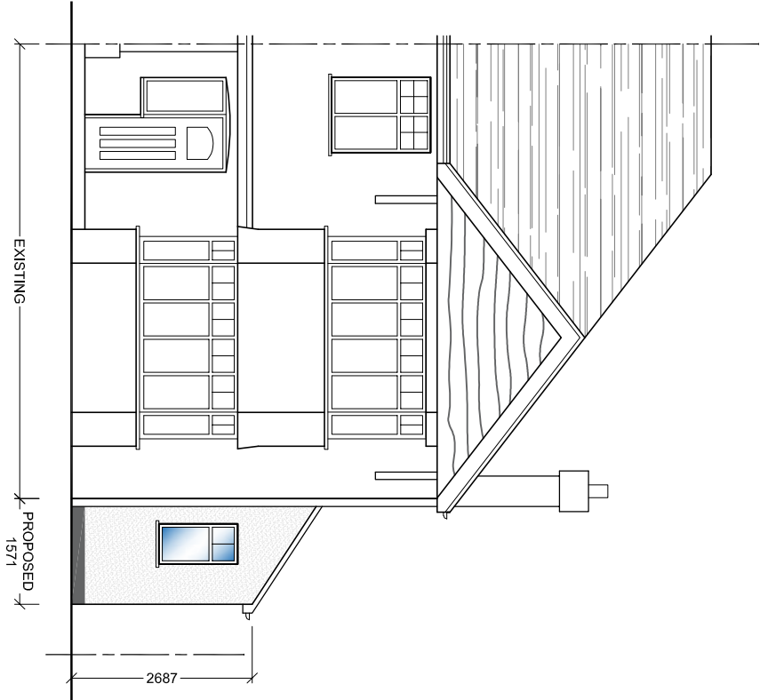
SOUTH ELEVATION
